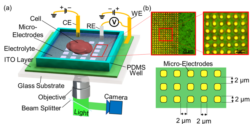
Figure 1. (a) Illustration of the method for rapid surface charge mapping. WE, RE, and CE are working, reference, and counter electrodes, respectively. The incident light illuminates the ITO layer from the backside. A cell sits on the surface of a microelectrode array. The local surface charge of the cell induces a change in the photoelectric effect. A CCD camera is used to capture the reflected light. (b) Microscopic images and scheme of the microelectrode array.
