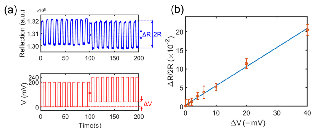
Figure 3. (a) Reflection intensity of a microelectrode with the changing of the applied voltage V = V_w - V_{re} , which is the voltage difference between the working and reference electrodes. The measurement was conducted in DI water. (b) The normalized reflection intensity changes as a function of the modulation amplitude \Delta V .
