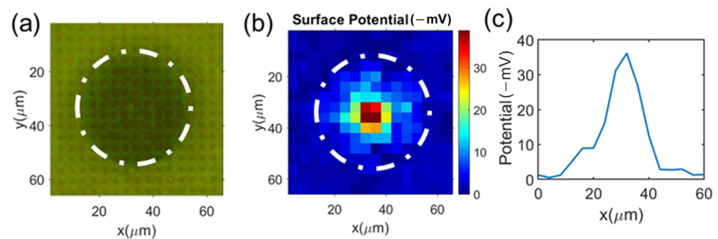
Figure 4. (a) Optical image (top illumination) of an MP sitting on the microelectrode array surface; (b) surface charge mapping measurement of this single MP using the microelectrode array; and (c) the profile of the measured surface electrical potential along the center line in the x-direction.
