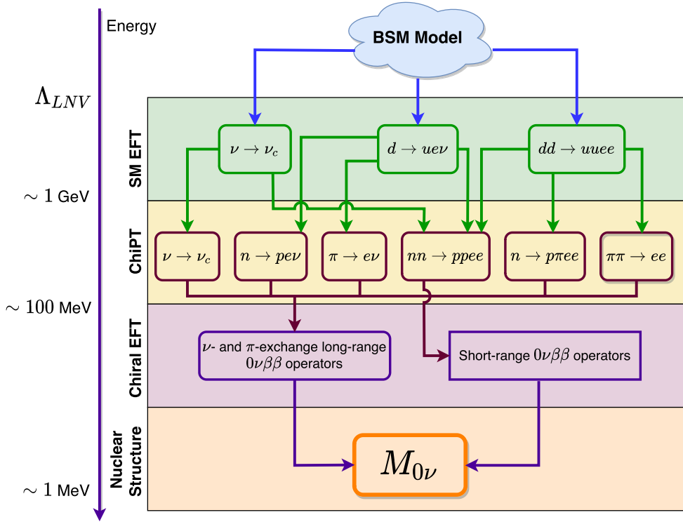
Figure 1. A ‘tower of theories’ leading to the computation of the nuclear matrix elements M_{0\nu} that control the rate of 0\nu\beta\beta decay. At the highest level, above the cutoff \Lambda_{LNV} for all effective theories, is the ultimate BSM LNV. It manifests itself at the quark and gluon level through Standard-Model EFT, at the nucleon and pion level through chiral perturbation theory (ChIPT), at the nucleon-only level (i.e. with pions no longer part of the Hilbert space, but instead accounted for in multi-nucleon operators) through chiral-EFT, and at the nuclear level through the techniques of nuclear-structure theory. Figure adapted from [27].
