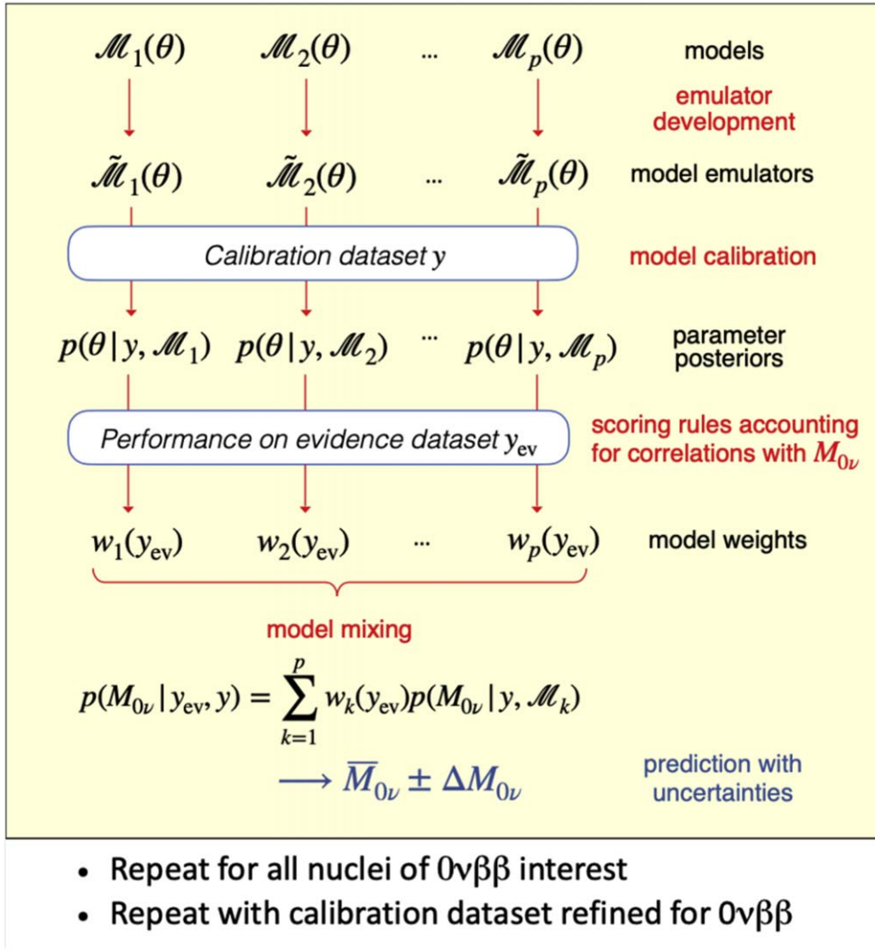
Figure 3. The road to calculations of M_{0\nu} with UQ that accounts for all limitations of the nuclear-physics calculation: truncation errors in chiral-EFT, uncertainties in the theory's parameters, and deficiencies of the many-body methods used. Emulator development is the first step, as it is key to facilitating subsequent calculations. Model parameters \theta can be calibrated against a dataset y . Weights for the different many-body methods will be obtained by assessing methods' performance on a set of observables \{y_{ev}\} . The weights w_k(y_{ev}) are to be computed via scoring rules that gauge predictive accuracy [162] and will also take account of the extent to which different members of \{y_{ev}\} are correlated with M_{0\nu} .
