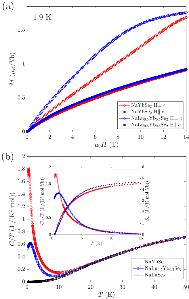
FIG. 4. (a) Magnetization of \text{NaLu}_{0.5}\text{Yb}_{0.5}\text{Se}_2 and \text{NaYbSe}_2 as a function of field, taken at 1.9 K in both cases. (b) Zero-field specific heat of both compounds, compared to the nonmagnetic analog \text{NaLuSe}_2 . The inset shows the magnetic specific heat and also the released entropy. The solid blue line is a fit of the \text{NaLu}_{0.5}\text{Yb}_{0.5}\text{Se}_2 data to a Gaussian broadened two-level system, and the dashed black line is at R \ln 2 , the upper bound for a spin-1/2 system.
