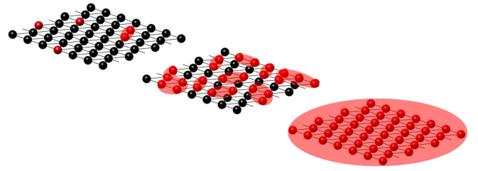
FIG. 5. Schematic to show the proposed evolution of correlations as a function of doping in \text{NaLu}_x\text{Yb}_{1-x}\text{Se}_2 , from isolated single ions and dimers ( x = 0.9 , left), through larger, finite magnetic clusters at the percolation threshold ( x = 0.5 , middle), to the full magnetic, many-body entangled state ( x = 0 , right).
