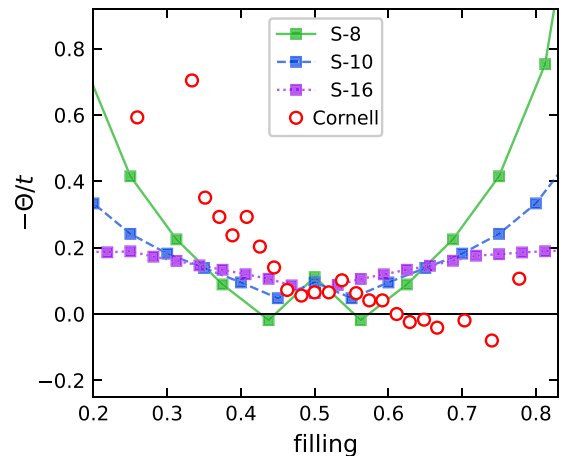
FIG. 7. Curie-Weiss temperature ( \Theta ) versus filling for the square-lattice Hubbard model with U/t = 20 (for three finite sizes) as compared to the Cornell experiment [9].
