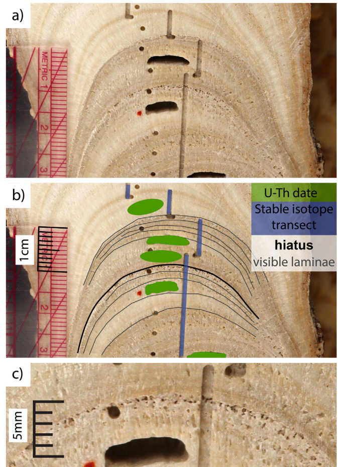
Fig. 4. Close-up of the Mid- to Late-Holocene hiatus in AK1. a) image with no annotation. b) image with annotation. Green shaded areas denote U–Th date sampling locations, blue shaded areas denote stable isotope transect trench, visible laminae in thin black lines, the Mid- to Late-Holocene hiatus in thick black line, unmarked circular pits are stable isotope drill holes from a low-resolution pilot study. c) higher zoom unannotated image of the Mid- to Late-Holocene hiatus.
