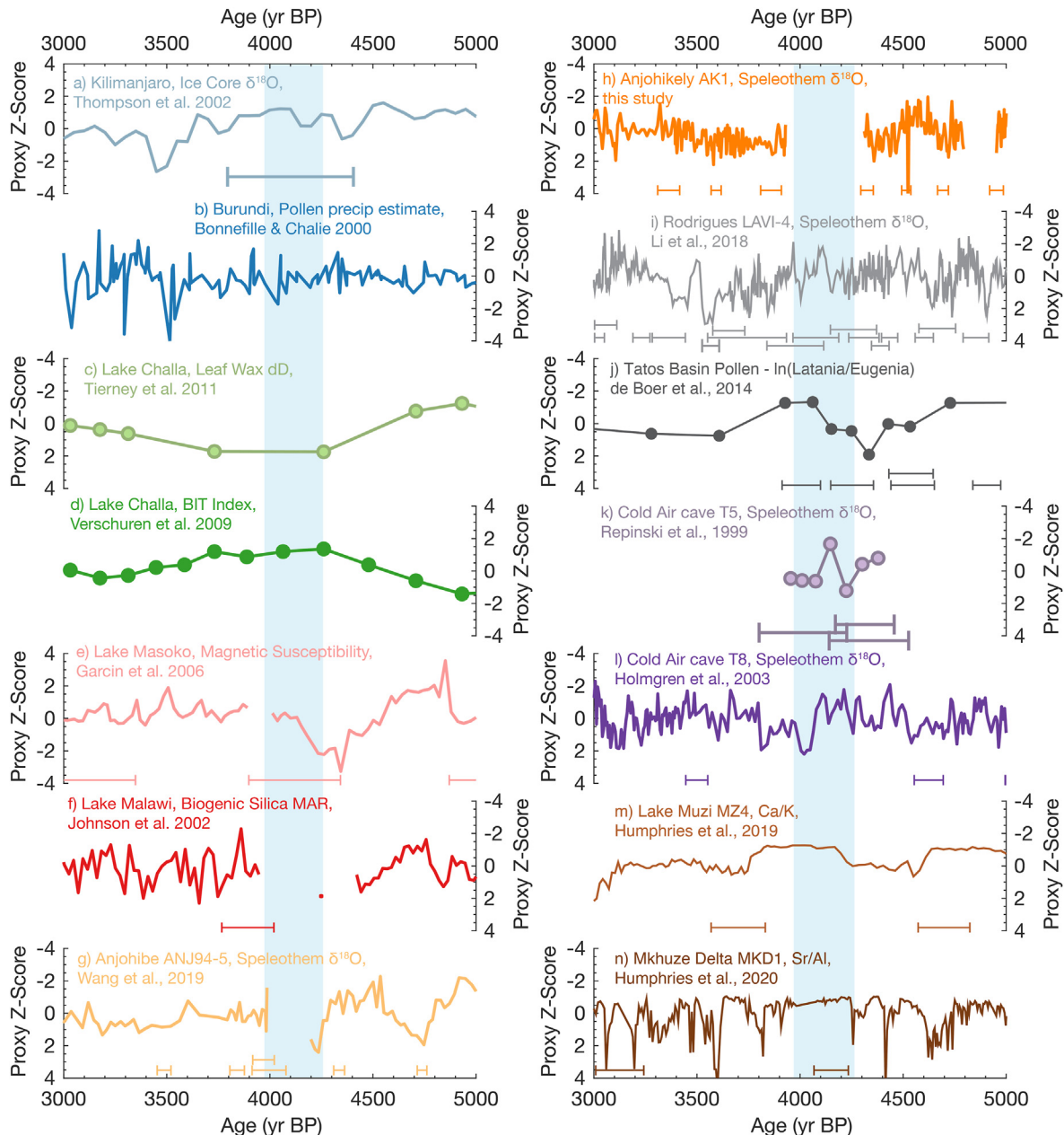
Fig. 6. Regional hydroclimate changes in southeast Africa between 5 and 3 kyr BP. For each record proxy z-score is calculated between 2.5 and 5.5 kyr BP to reduce the influence of orbital scale changes. Circles indicate datapoints. Lines without circles are at higher resolution so circles have been omitted for clarity. Error bars show radiocarbon or U–Th dates for each record and errors. Blue bars indicate the duration of the 4.2 ka event. Records are plotted so that wet conditions are consistently up.
