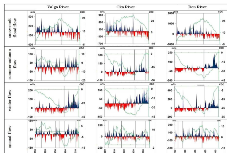
Figure 2. Long-term changes in snowmelt flood flow, summer–autumn water flow, winter water flow, and mean annual water flow in the Volga River at Staritsa, the Oka River at Kaluga, and the Don River at Stanitsa Kazanskaya. Blue and red fields indicate positive and negative deviations relative to long-term averages, respectively; the green line is the normalized cumulative deviation curve (CDC). The vertical black lines show phase boundaries (shift points) of increased or decreased values of the water flow.
