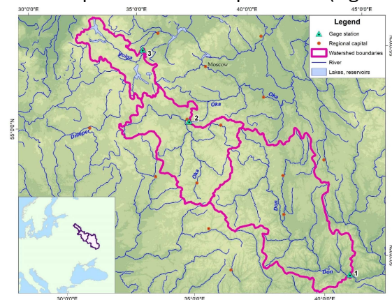
Figure 1. Three studied upstream river basins and river gauge locations at their closures. 1—the Don River at Stanitsa Kazanskaya, 2—the Oka River at Kaluga, 3—the Volga River at Staritsa. Major map projection is Lambert Azimuthal Equal Area projection (central meridian 20 E, latitude of origin 45 N).
