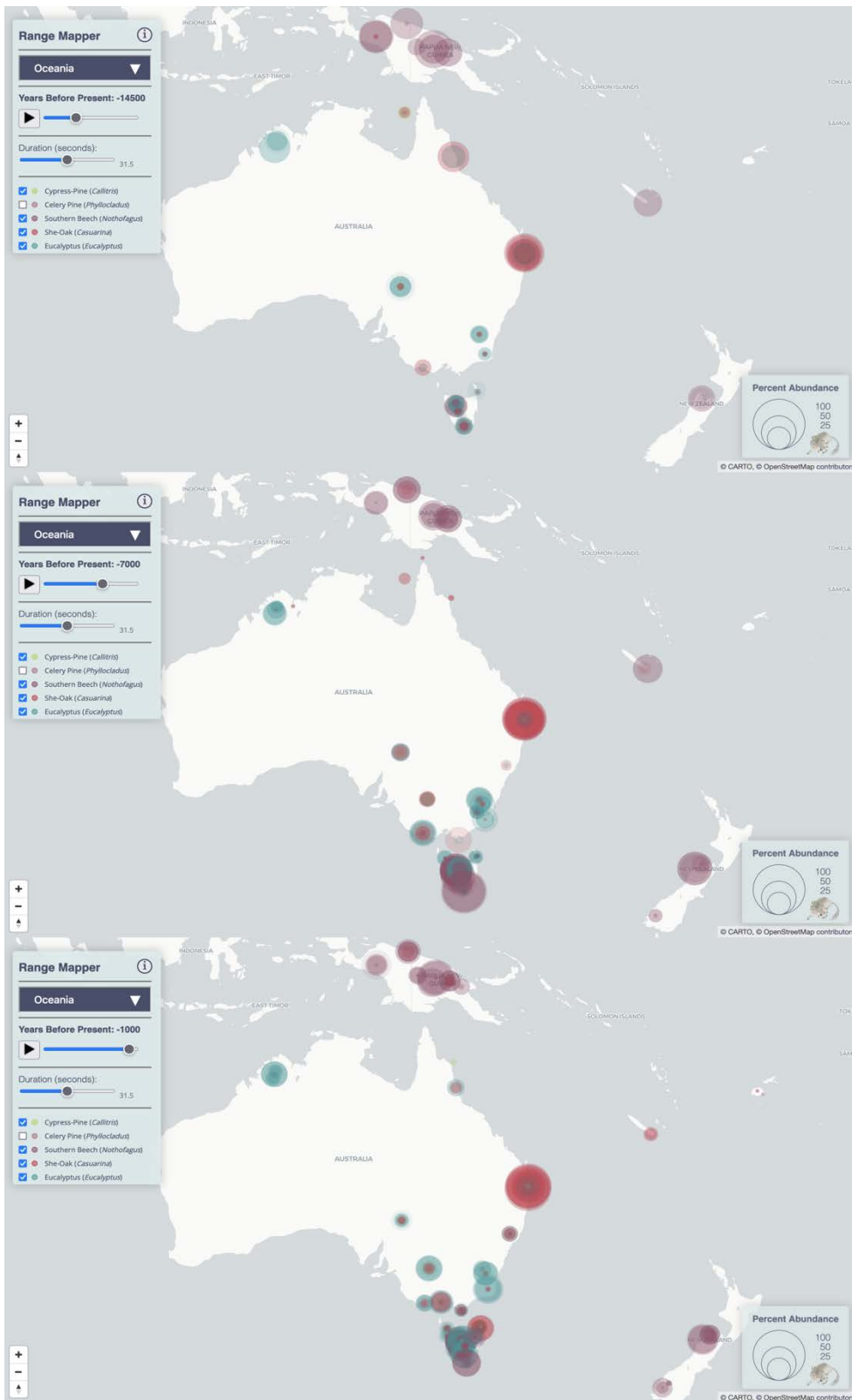
Figure 6: Range Mapper screenshots of Oceania from 14.5, 7, and 1 ka BP. While Neotoma data for Oceania are still relatively sparse, phenomena such as the early Holocene expansion of Eucalyptus and Nothofagus in Tasmania can be seen.
