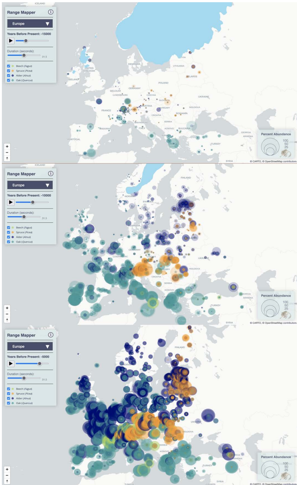
Figure 4: Range Mapper screenshots of Europe from 15, 10, and 5 ka BP. Four iconic tree taxa are shown here: beech ( Fagus ), spruce ( Picea ), alder ( Alnus ) and oak ( Quercus ). Vegetation changes shown by Range Mapper include the known glacial refugia, the post-glacial expansion of beech, rapid range expansion of oak at the onset of Holocene warming, and the late Holocene expansion and westward shifts of spruce and beech population centers.
