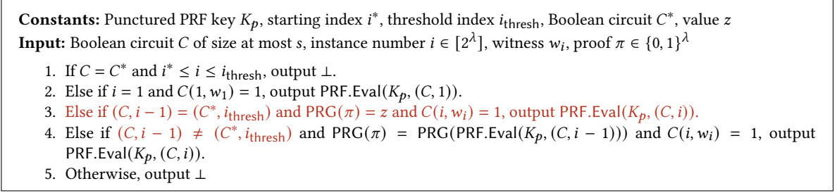
Figure 5: Program \text{Prove}''[K_p, i^*, i_{\text{thresh}}, C^*, z]
