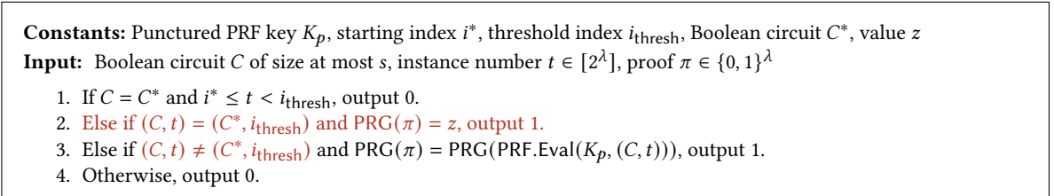
Figure 6: Program \text{Verify}''[K_p, i^*, i_{\text{thresh}}, C^*, z]
