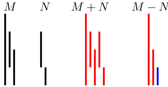
■ Figure 5 Illustration of the barcodes for M, N \in \mathbf{Pvec} and M+N, M-N \in \mathbf{SPvec} . For M+N and M-N , a red interval is positively signed and a blue interval is negatively signed.
