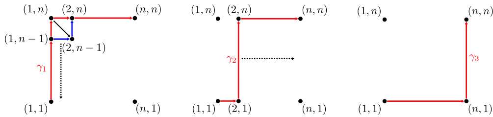
■ Figure 6 We start with \gamma_1 on the left, and then push \gamma_1 through the square to track along the lower-right corner of the square (in blue). We repeat this process, descending down each square in the first column until we reach \gamma_2 (middle). Then we repeat this process column-by-column until we've reached \gamma_n (right).
