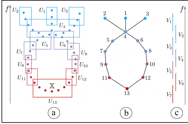
Figure 1. A simple example of computing a mapper graph. A point cloud \mathbb{X} in (a) is colored by the height (e.g. y-coordinate) function f : \mathbb{X} \rightarrow \mathbb{R} . The cover \mathcal{U} = U_1, \dots, U_{13} of \mathbb{X} is induced by a cover \mathcal{V} = \{V_1, \dots, V_7\} of f(\mathbb{X}) that contains 7 intervals with 1/3 overlap in (c). The 1-dimensional nerve of \mathcal{U} is the mapper graph in (b).
