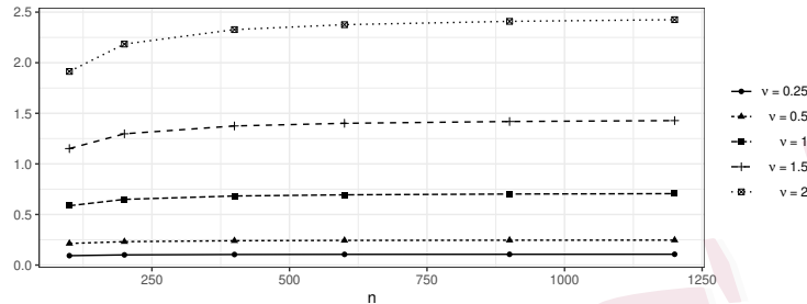
Figure 1: Trend of \sum_{i=1}^n E_1(e_{i,1} - e_{i,0})^2 / E_1 e_{i,1}^2 for Matérn model when \chi is a regular grid \chi = \{i\delta : 0 \leq i \leq n\} . Parameter \sigma^2 in Matérn covariogram equals 1.0 and decay \phi for different \nu are set to make the correlation of two points equals 0.05 when their distance reaches 0.2.
