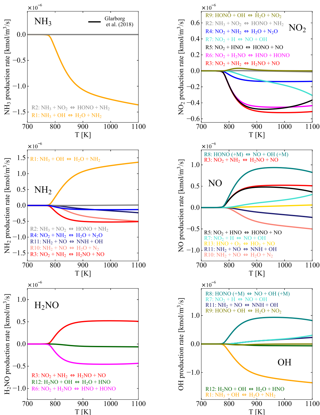
Fig. 4. Rate of production [kmol/m³/s] of NH 3 , NO 2 , NH 2 , NO, H 2 NO, and OH generated using the model of Glarborg et al. [41].
