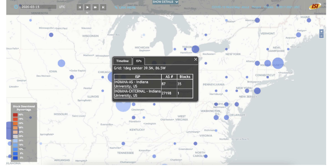
Fig. 8. Discovered using the ISP drill-down tables, central Indiana experienced its largest downtrend on 2020-03-15 due to Indiana University ending classes for spring break (see Section IV-C).
