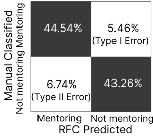
Figure 3: Confusion Matrix.
