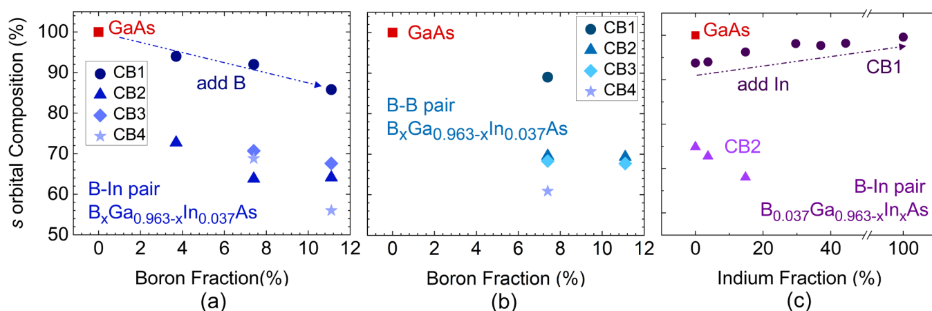
FIG. 7. s orbital composition of CB states near zone center: (a) for B–In pair B_xGa_{0.963-x}In_{0.037}As , x = 0.037 – 0.111 ; (b) for B–B pair B_xGa_{0.963-x}In_{0.037}As , x = 0.074 – 0.111 ; and (c) for B–In pair B_{0.037}Ga_{0.963-x}In_xAs , x = 0 – 0.444 .
