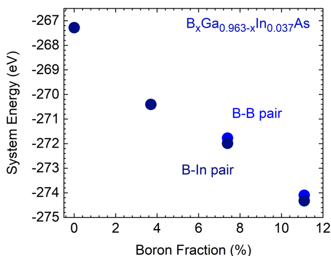
FIG. 2. Ground state system energy for B–B pair and B–In pair configurations for various fractions of B in B_xGa_{0.963-x}In_{0.037}As .
