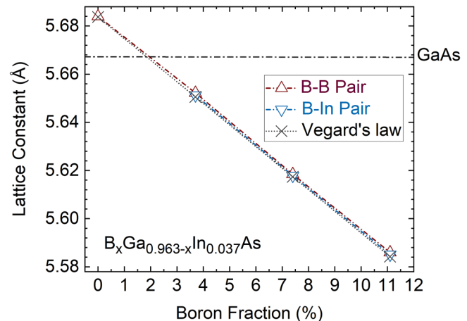
FIG. 3. Lattice constant in B_xGa_{0.963-x}In_{0.037}As for B-B pair and B-In pair configuration when adding B compared with lattice constant calculated using Vegard's law. GaAs dash-dotted line is calculated from VASP. Lines are a guide to the eye.
