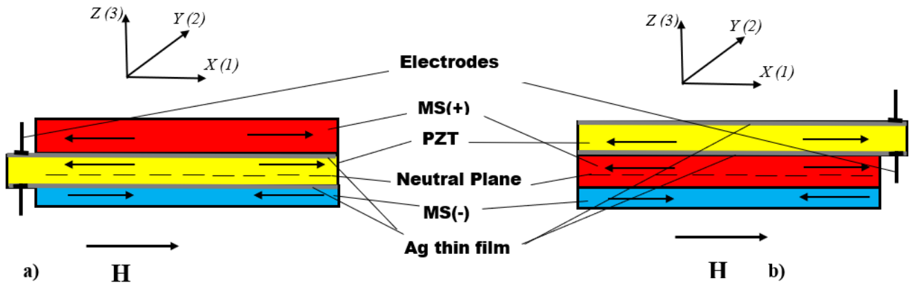
Fig. 1 Schematic drawing of (a) Type 1 and (b) Type 2 asymmetric trilayers, with PZT layer of thickness t^p and magnetostrictive (MS) layers with positive (MS+) and negative (MS-) magnetostriction and thicknesses t^{m1} and t^{m2} respectively. The dashed line represents the neutral plane.
