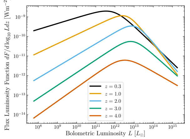
FIG. 1: The flux distribution of AGN as a function of an AGN's bolometric luminosity at redshifts z \in \{0.3, 1.0, 2.0, 3.0, 4.0\} , as given by Eq. (8).
