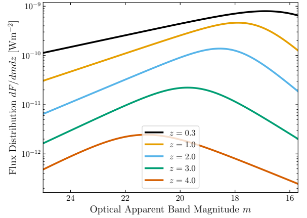
FIG. 2: The flux distribution of AGN as a function of an AGN's apparent magnitude in an optical band b at redshifts z \in \{0.3, 1.0, 2.0, 3.0, 4.0\} , as given by Eq. (9). In order to show the full range of this distribution, we do not include the theta function factor.
