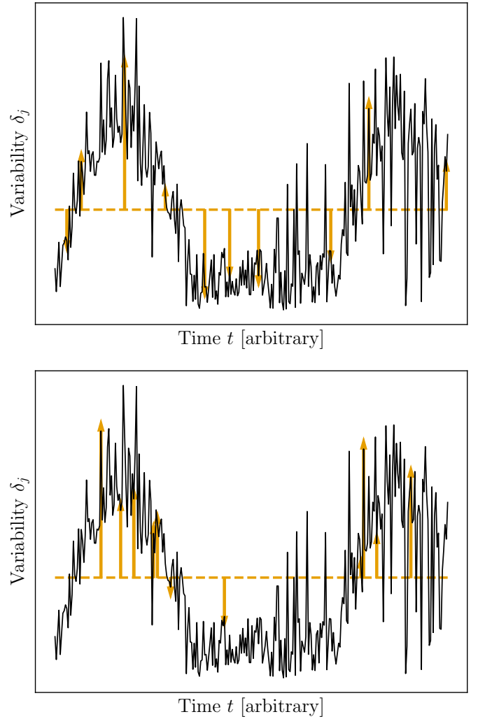
FIG. 4: An example of the variability \delta_j(t) of AGN j shown in solid black, plotted against the variability \delta_j(t_\alpha) evaluated at the neutrino arrival times t_\alpha , depicted by solid orange arrows. The dashed orange line indicates the zero point, \delta_j = 0 . In the top figure the neutrinos arrive randomly, and thus a cross correlation between these two quantities would become zero. In the bottom figure the neutrinos are sourced from AGN and thus are biased towards appearing when the intensity is higher, leading to nonzero correlation.
