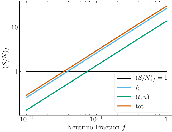
FIG. 5: The signal-to-noise ratio (S/N)_f for measuring the HEAN neutrino fraction f using both temporal and spatial data from VRO’s i band, IceCube, KM3NeT, and Baikal-GVD. Since pure spatial correlation dominates the SNR, the result is not very sensitive to the underlying AGN variability parameters. IceCube contributes \sim 8\% of the total SNR, while KM3NeT and Baikal-GVD each give \sim 46\% .
