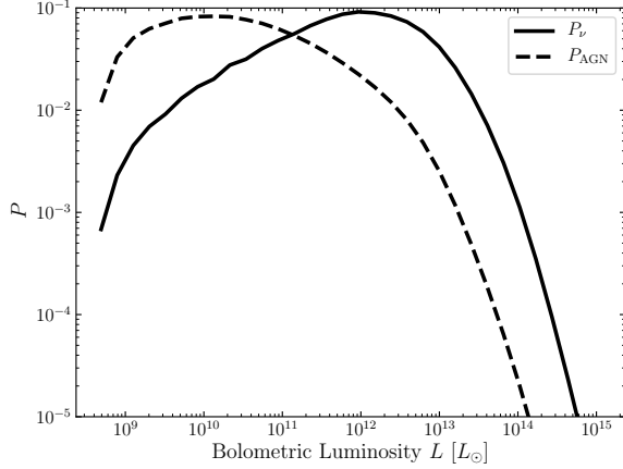
FIG. 3: The observation probability P associated with neutrinos and AGN in each bolometric luminosity bin between redshifts 0.3 \leq z \leq 6.7 . Over the range of luminosities presented, 33 base-10 logarithmic bins are taken. The solid black line is the probability that an AGN emitting neutrinos has bolometric luminosity L , while the dashed black line is the probability of that an observed AGN has bolometric luminosity L . Both curves are normalized by the set of observed AGN and are computed assuming a limiting magnitude of m_{\text{lim}} = 24.0 . At large luminosities both curves follow the expected flux distribution curve of Fig. 1, however at small L the limiting magnitude restricts the total number of AGN observed.
