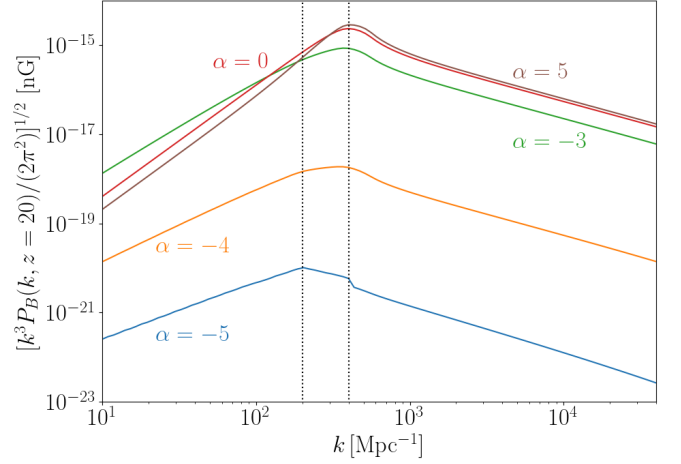
FIG. 2. The magnetic-field power spectrum as a function of wavenumber for different values of the electron-density spectral index \alpha . For values of \alpha > -3 ( \alpha \leq -3 ), the normalization of the CIP power spectrum is taken to be the maximum allowed by the BBN (CMB) constraint, Eq. (3) (Eq. (5)). The vertical lines indicate the assumed Jeans wavenumber k_J = 200 \text{ Mpc}^{-1} and the cutoff k_{\max} = 400 \text{ Mpc}^{-1} in the electron-density power spectrum.
