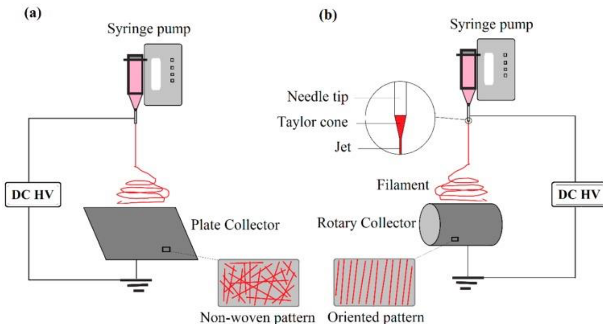
Figure 6. A typical electrospinning set up [130] using (a) a static grounded collector plate and (b) a grounded rotating drum collector. Reprinted from Ref. [130], available at https://doi.org/10.3390/ma10111238 ; accessed on 1 December 2022.
