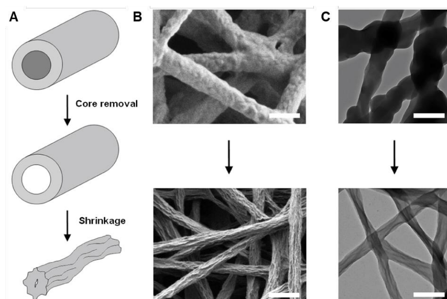
Figure 14. Polyvinylpyrrolidone electrospun with ferric tosylate and coated with PEDOT is rinsed with methanol to form hollow PEDOT nanofibers that collapse somewhat and fuse together [186]. (A) Process upon rinsing with methanol. (B) SEM and (C) TEM of the nanofibers. All scale bars represent 1 \mu\text{m} . Reprinted with permission from Ref. [186].
