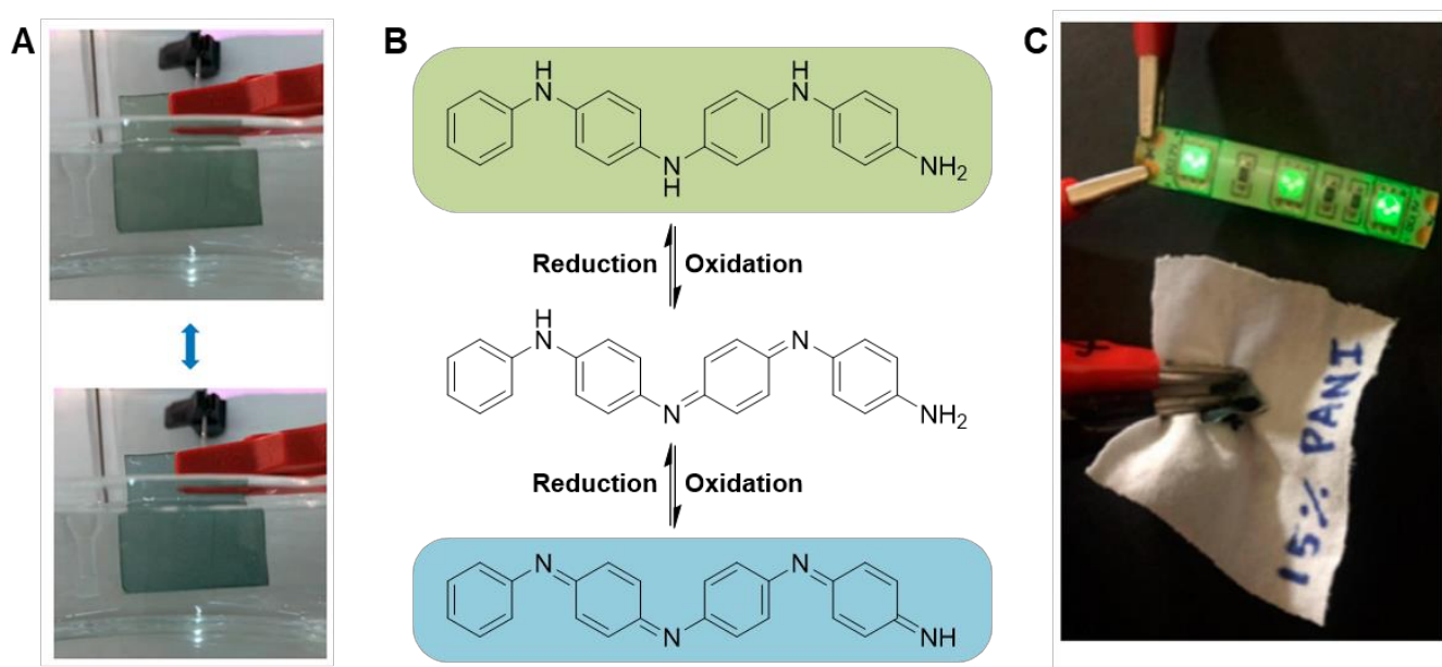
Figure 26. Electrochromic and conductive property exhibited by electrospun PANI/silk fibroin nanofibers [239]: (A) green coloration observed on PANI/silk fibroin after the application of 0.2 V and blue coloration observed after application of 0.6 V; (B) schematic of the structural and color changes accompanying the oxidation and reduction of PANI; (C) the same PANI/silk fibroin nanofibers sewn onto cotton fabric and used as a conductor to light up LEDs. Reprinted with Ref. [239], available at https://doi.org/10.3390/polym12092102 , accessed on 1 December 2022.
