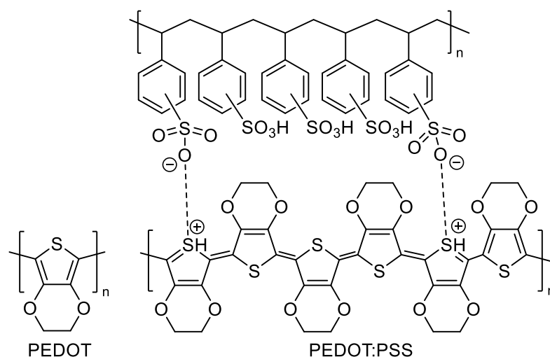
Figure 5. Left: Structure of poly(3,4-ethylenedioxythiophene) (PEDOT); Right: structure of PEDOT:PSS.
