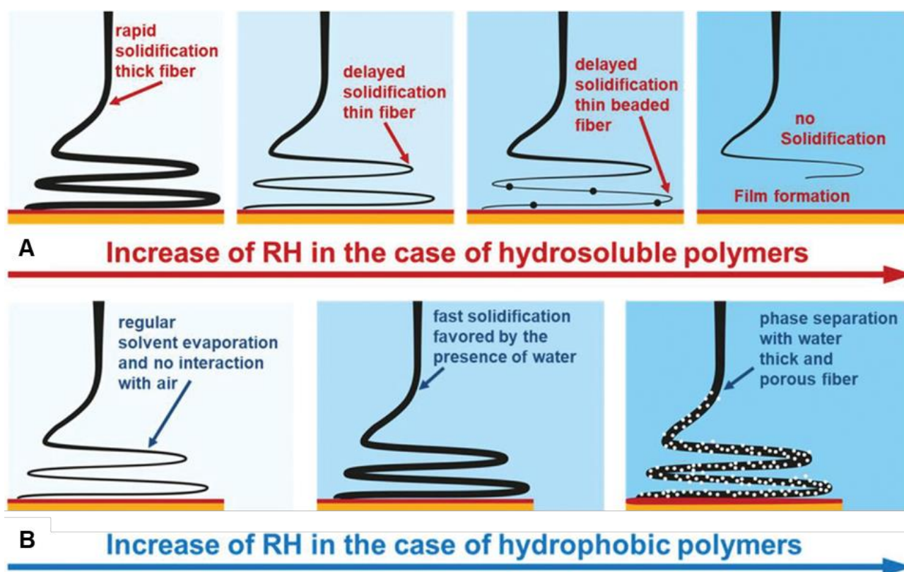
Figure 10. Effect of increasing relative humidity (RH) on (A) water-soluble and (B) hydrophobic electrospun polymers. Reprinted from [168]. Copyright 2021, John Wiley & Sons.
