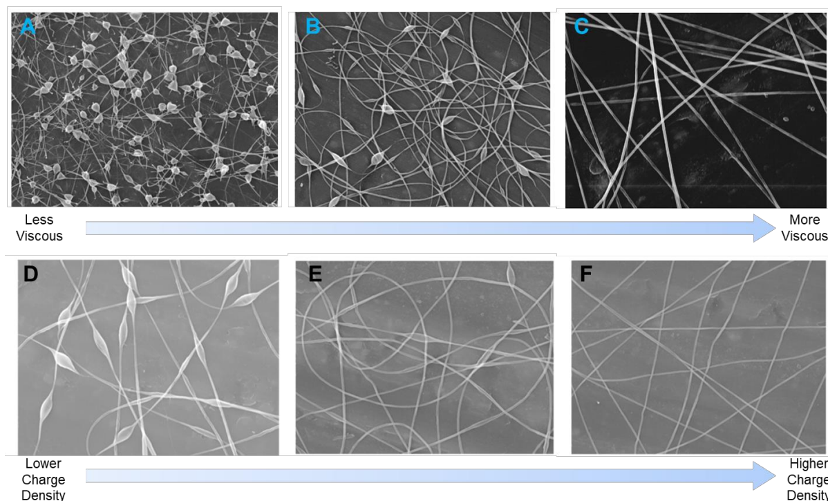
Figure 7. Increasing viscosity or conductivity (charge density) reduces bead formation [135]. Top: Scanning electron micrographs (SEMs) of electrospun aqueous poly(ethylene oxide) (PEO). The horizontal edge of each image is 20 \mu\text{m} long: (A) 1.5 wt.% PEO, 32 cP; (B) 3 wt.% PEO, 289 cP; (C) 4 wt.% PEO, 1250 cP. Bottom: Electrospun 3 wt.% PEO with increasing NaCl content: (D) 15 ppm NaCl, 1.23 \text{C}\cdot\text{L}^{-1} ; (E) 300 ppm NaCl, 3.03 \text{C}\cdot\text{L}^{-1} ; (F) 1500 ppm NaCl, 28.8 \text{C}\cdot\text{L}^{-1} . Reprinted from Ref. [135], Copyright 1999, with permission from Elsevier.
