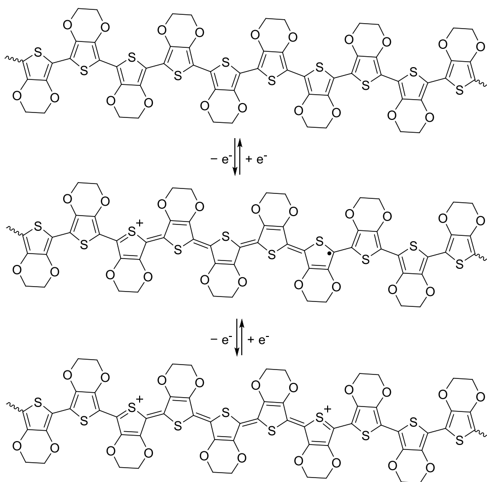
Figure 3. Reversible oxidation and reduction processes form resonance-delocalized electrons and cations (holes) along the backbone of CPs such as PEDOT. Redox processes, which are typically reversible, allow interconversion among neutral polymers ( top ), radical cations known as polarons ( middle ), and dications known as bipolarons ( bottom ). Reprinted from Ref. [45], available at https://www.mdpi.com/1996-1944/12/16/2629 ; accessed on 1 December 2022.
