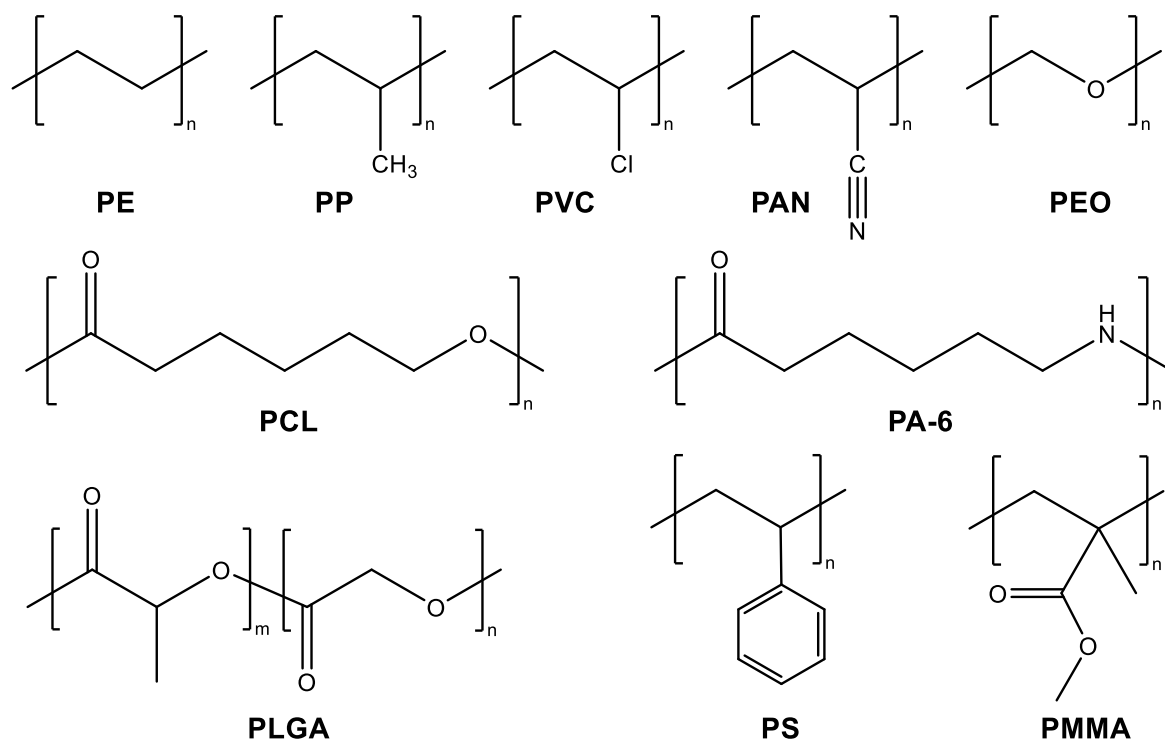
Figure 8. Synthetic polymers commonly used for electrospinning include: polyethylene (PE), polypropylene (PP), poly(vinyl chloride) (PVC), poly(acrylonitrile) (PAN), poly(ethylene oxide) (PEO), polycaprolactone (PCL), polycaprolactam (also known as nylon 6 and polyamide 6, PA-6), poly(lactic-co-glycolic acid) (PLGA), polystyrene (PS), and poly(methyl methacrylate) (PMMA).
