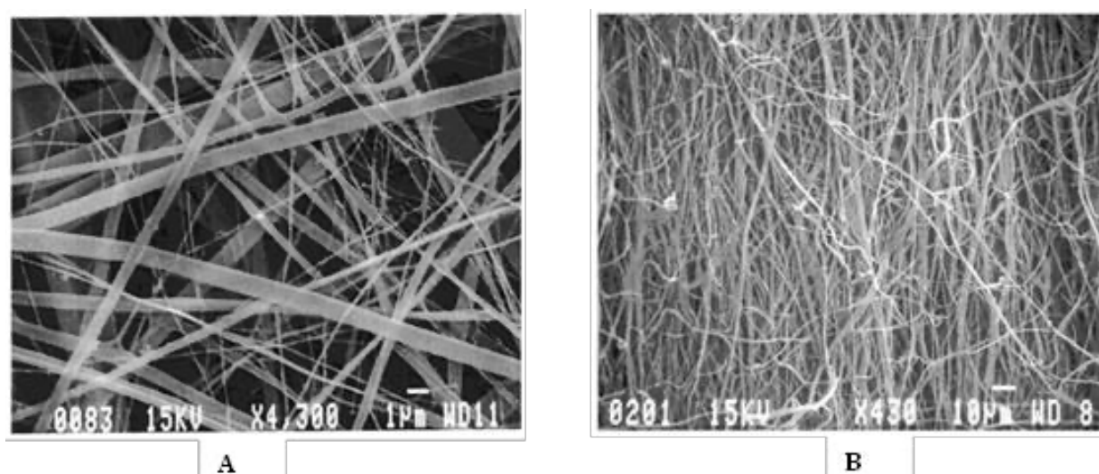
Figure 9. SEMs of electrospun collagen [157]. (A) Randomly oriented fibrils generated at less than 500 rpm. (B) Aligned fibrils generated at 4500 rpm. Reprinted and adapted with permission from [157]. Copyright 2002, American Chemical Society.
