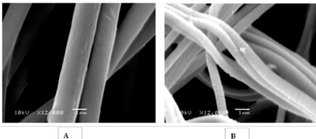
Figure 12. SEMs of (A) core–sheath PANI/PMMA electrospun nanofibers and (B) electrospun PANI nanofibers after removal of PMMA [182]. Reprinted with permission from Ref. [182]. Copyright 2012.
