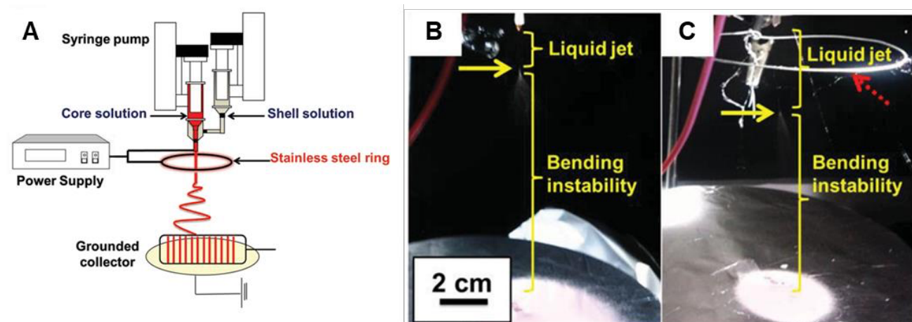
Figure 19. Use of a secondary electric field below the syringe (A) results in prolonged liquid jets (B,C) that enhance charge transport, resulting in dramatically enhanced mobility [200]. Reprinted with permission from Ref. [200]. Copyright 2015, John Wiley & Sons.
