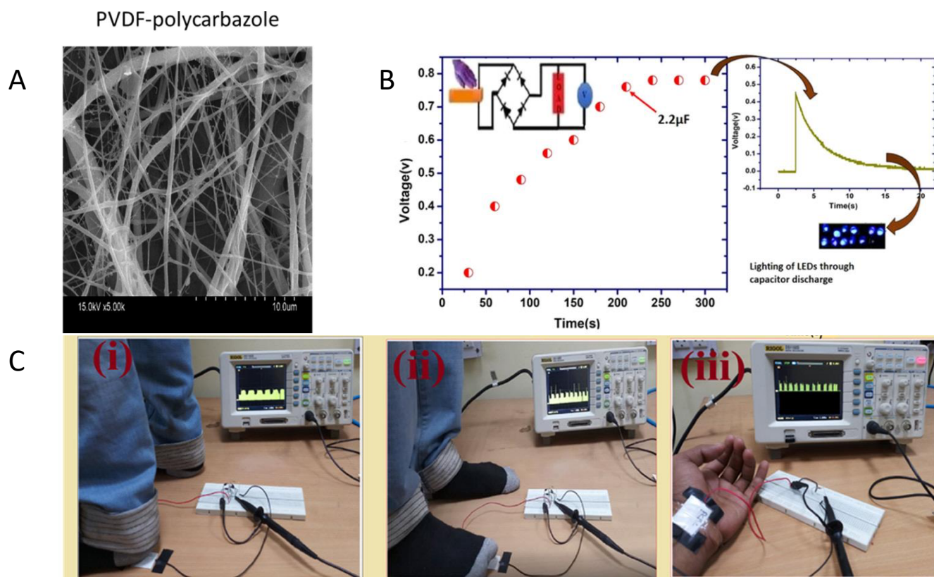
Figure 24. Energy-harvesting device constructed from PVDF–PCZ [235]: (A) SEM image of PVDF–PCZ nanofibers; (B) voltage measurements of the PVDF–PCZ nanocomposite showing the charging of a capacitor, and subsequent illumination of five LEDs after discharging; (C) types of human motion that generated voltage in the nanocomposite: (i) heel movement, (ii) toe movement, and (iii) wrist bending. Reprinted with permission from [235]. Copyright 2021, American Chemical Society.
