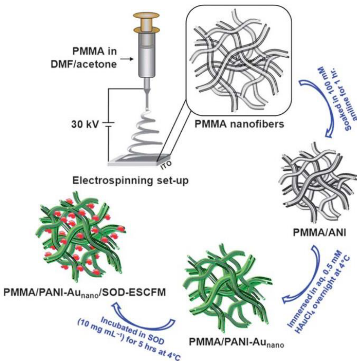
Figure 20. PMMA/PANI superoxide sensors were prepared by electrospinning PMMA and coating the resultant nanofibers with PANI via chemical oxidation of aniline with hydrogen tetrachloroaurate [261]. The enzyme superoxide dismutase was then bonded to the gold nanoparticles formed in the PANI during oxidation, and the enzyme was used to detect superoxide. Republished with permission of Ref. [261]; permission conveyed through Copyright Clearance Center, Inc.
