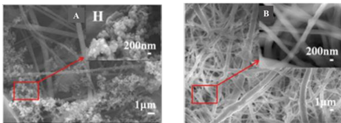
Figure 13. SEMs of (A) cellulose/PNVPy coated nanofibers and (B) cellulose/P3HT-coated nanofibers [245]. Republished with permission from Ref. [245], Permission conveyed through Copyright Clearance Center Inc.
