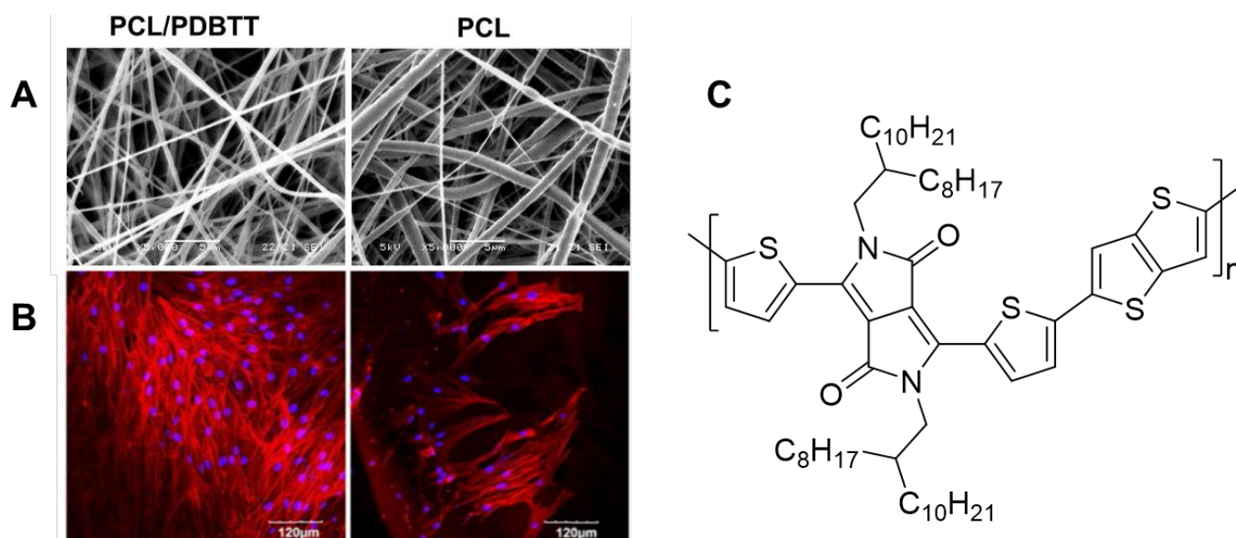
Figure 15. Wound healing application of electrospun CPs [204]: (A) SEM images of electrospun PCL/PDBTT and PCL nanofibers; (B) confocal and SEM images of extent of growth of HDF on electrospun PCL/PDBTT and PCL nanofibers, showing enhanced HDF growth on PCL/PDBTT with light stimulation; (C) structure of thiophene/pyrrole-based polymer PDBTT. Reprinted with permission from Ref. [204]. Copyright 2017, with permission from Elsevier.
