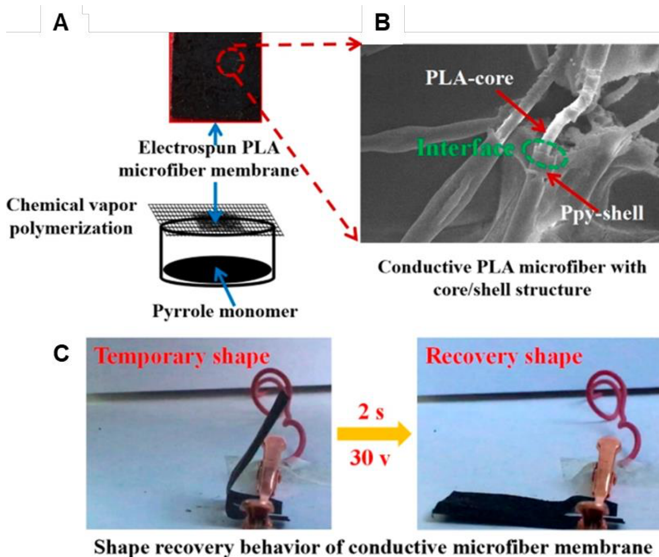
Figure 25. Shape memory device constructed from PPy coated on electrospun PLA [277]: (A) schematic of in situ polymerization of PPy onto electrospun PLA; (B) SEM image showing core/shell structure of nanocomposite with PLA as the core and PPy as the shell; (C) effect of application and removal of 30 V across composite resulting from the conduction of a heat-generating electric current. Reprinted with permission from [277]. Copyright 2018, American Chemical Society.
