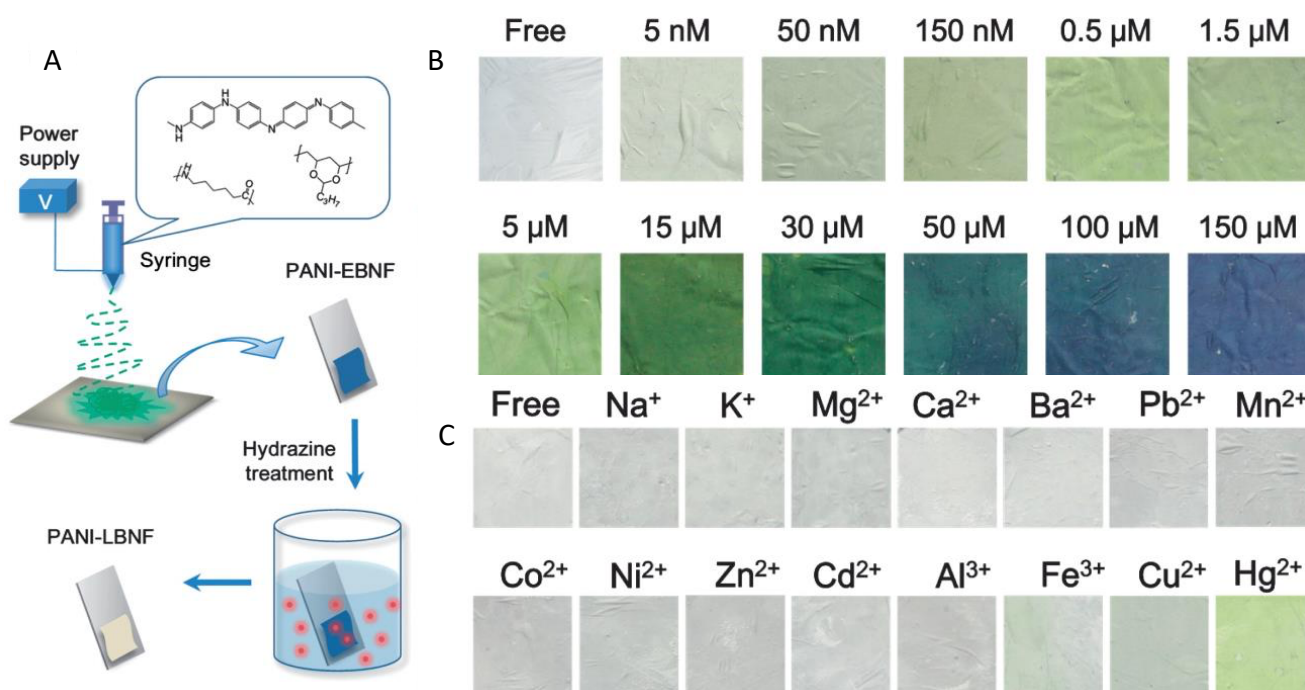
Figure 21. PANI-containing electrospun composite used for colorimetric sensing of Hg(II): (A) process for synthesis of PANI sensor strip showing electrospinning of a mixture of PANI, polyvinylbutyral, and poly(amide-6) and then treatment with hydrazine; (B) result of incubating PANI sensor strip in Hg(II) aqueous solutions showing progressive discoloration and darkening after contact with increasing Hg(II) concentration; (C) sensor strip after incubation in solutions of different metals, showing selectivity of sensing to Hg(II). Republished with permission of The Royal Society of Chemistry from [227]; permission conveyed through Copyright Clearance Center, Inc.
