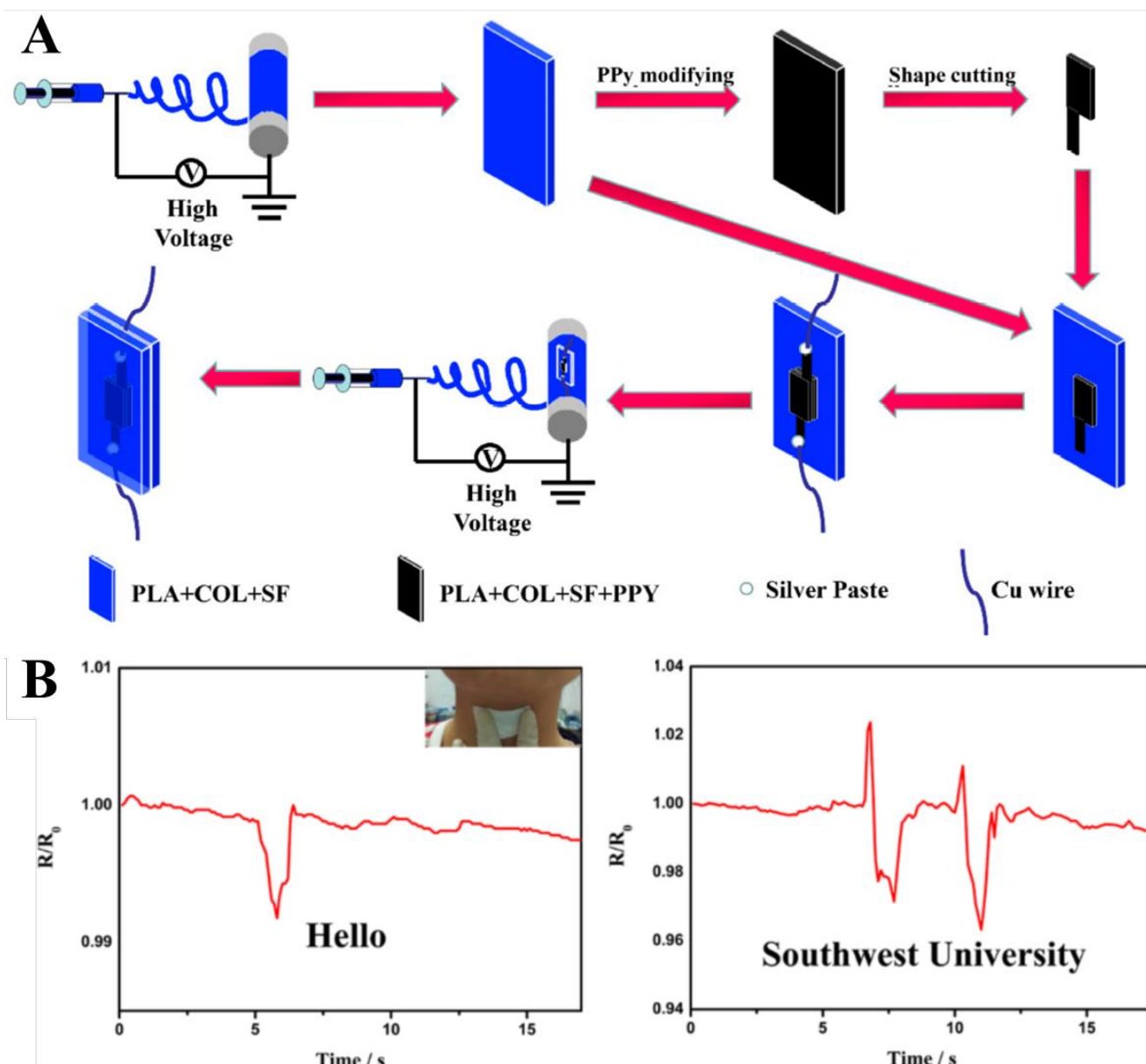
Figure 23. Human motions detectable by a piezoresistive sensing device composed of PPy-coated PLA/silk fibroin/collagen [268]: (A) fabrication via PPy coating of electrospun PLA/silk fibroin-collagen nanofibers; (B) vocal cord vibrations detected by a change in resistance in the sensor. Reprinted from [268], available at https://doi.org/10.3390/polym10060575 , accessed on 1 December 2022.
