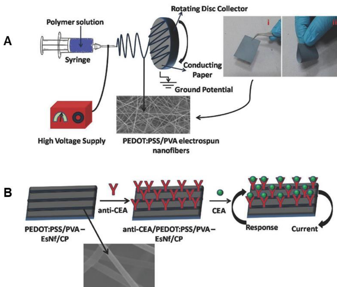
Figure 22. Biosensor developed from PEDOT:PSS/PVA to detect carcinoembryonic antigen (CEA) [230]: (A) diagram of electrospinning setup of PEDOT:PSS/PVA nanofibers; (B) schematic diagram of PEDOT:PSS/PVA-electrospun nanofibers/conducting paper and immobilization of CEA antigen. Reprinted from [230]. Copyright 2016, John Wiley & Sons.
