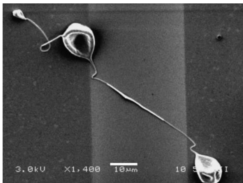
Figure 11. SEM showing a neat electrospun P3HT nanofiber having an average length of 54 \mu\text{m} and diameter of 670 nm [176]. Reprinted with permission from Ref. [176]. Copyright 2005 with permission from Elsevier.
