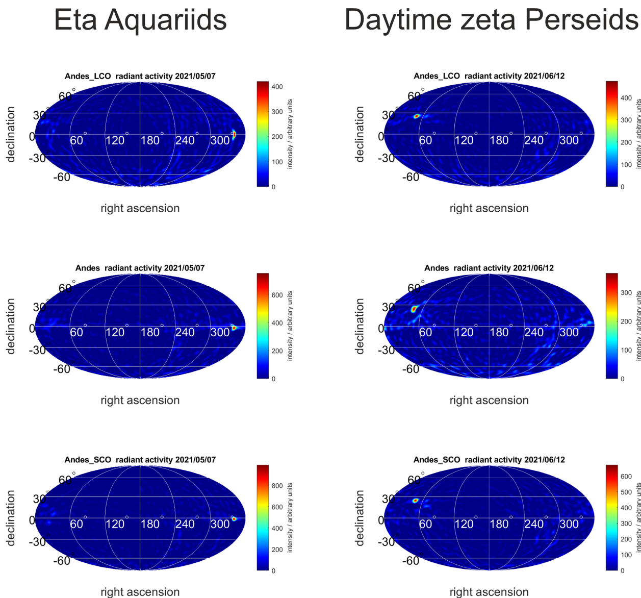
Figure 4. Meteor radiant activity maps derived from CONDOR for LCO, ALO (Andes), and SCO (the top, middle, and bottom row, respectively). The left column shows the source radiant activity for the \eta Aquariids, and the right panels present the daytime zeta Perseids. The meteor showers are identified from the catalogues presented in Brown et al. (2010) and Janches et al. (2013).
