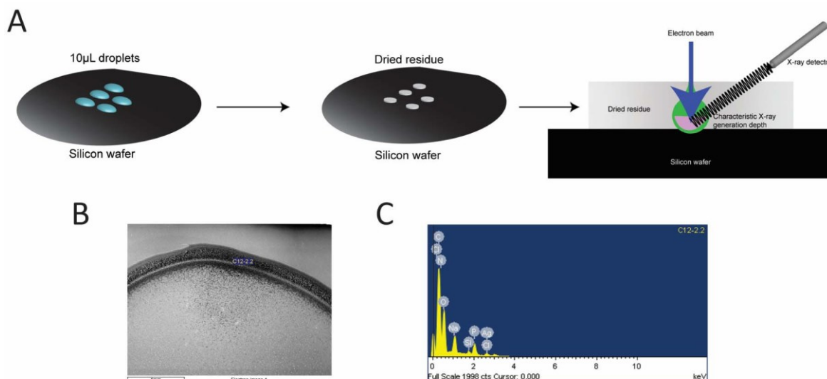
Fig. 3 (A) The general workflow for the SEM and EDS experiments. Purified solution of AgNC@hpC 12 is dried at ambient conditions on the silicon wafer under controlled humidity. (B) A representative SEM image of AgNC@hpC 12 samples and (C) the raw EDS spectrum of the same sample.
