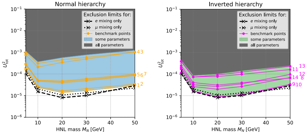
Figure 11. Original (black lines) and reinterpreted (colored lines) 95% exclusion limits on the total mixing angle U_{\text{tot}}^2 = \sum_{\alpha=e,\mu,\tau} \sum_{I=1,2} |\Theta_{\alpha I}|^2 for the normal (left) and inverted (right) mass orderings, for Majorana HNLs. The black lines are limits obtained under the single-flavor assumption. The solid colored lines denote those obtained for various benchmark points (defined in figure 2 from [407]) spanning the allowed regions shown in figure 3. When scanning over all ratios of mixing angles allowed by neutrino oscillation data, the exclusion limits span the blue (green) shaded regions. Correspondingly, the gray filled area is excluded at CL > 95% for all possible ratios of mixing angles, and thus constitutes an exclusion limit independent of the specific choice of mixing angles, valid as long as we consider the two HNL model explaining neutrino oscillations.
