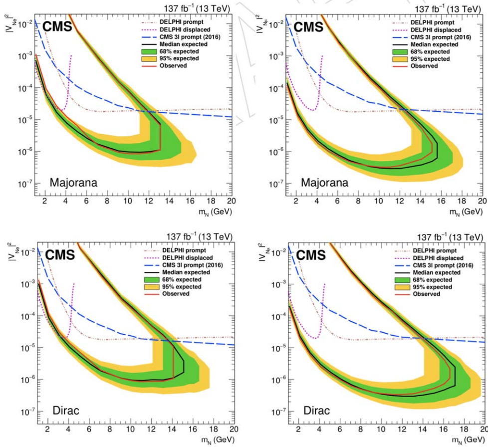
Figure 8. The 95% CL limits by the CMS experiment on |V_{eN}|^2 (left) and |V_{μN}|^2 (right) as functions of mass m_N for a Majorana (top) and Dirac (bottom) HNL. The area inside the red (black) curve indicates the observed (expected) exclusion region [409]. Previous results from the DELPHI and the CMS Collaborations (2016) are shown for reference.
