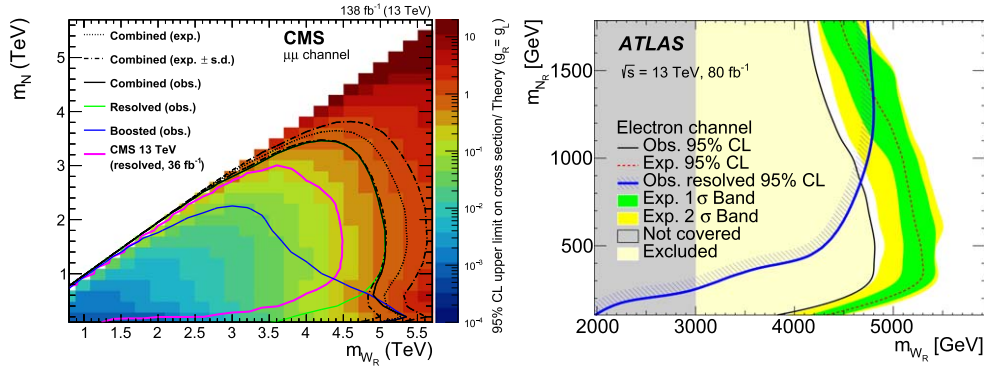
Figure 9. Left: the 95% CL limit with 138 fb -1 of data from CMS [427] on M_{W_R} and m_N in the \mu - \mu channels (resolved and boosted); similar bounds apply to the electron channel, see [428] for the ATLAS search. Right: The 95% CL limit with 80 fb -1 of data from ATLAS [433] on M_{W_R} and m_N in the e - e channel (boosted); similar bounds apply to the muon channel.
