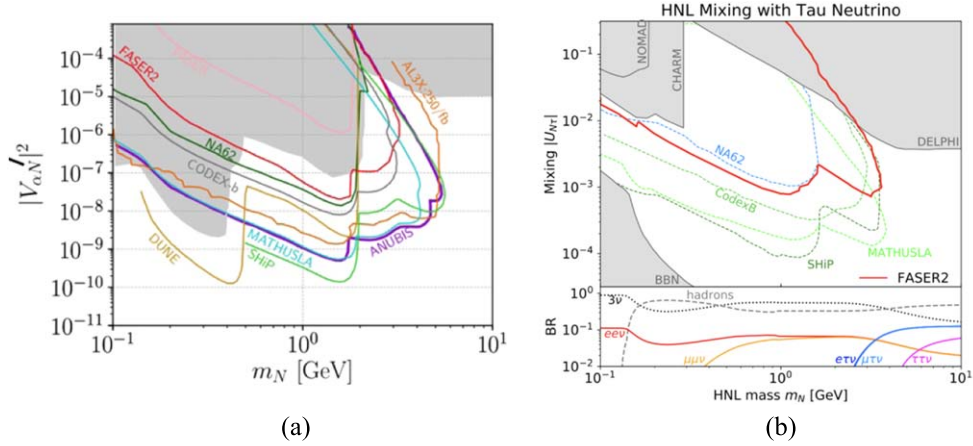
Figure 19. (left) ANUBIS/AL3X/MATHUSLA reach compared to other future experiments in the context of the minimal HNL scenario, with one generation of N mixing with either \nu_e or \nu_\mu but not both i.e. \alpha = e/\mu . Figure is taken from [483]. (right) Sensitivities for a HNL mixing with the tau neutrino in the (mass, coupling) plane. The sensitivity reaches of FASER2 are shown as solid red lines alongside existing constraints (dark gray-shaded regions) and projected sensitivities of other proposed searches and experiments (colorful dashed lines), as obtained in [484] [4, 31, 50, 91] and references therein. Figure is taken from [474, 485–487]. The top and bottom panels show the LLP’s branching fractions.
