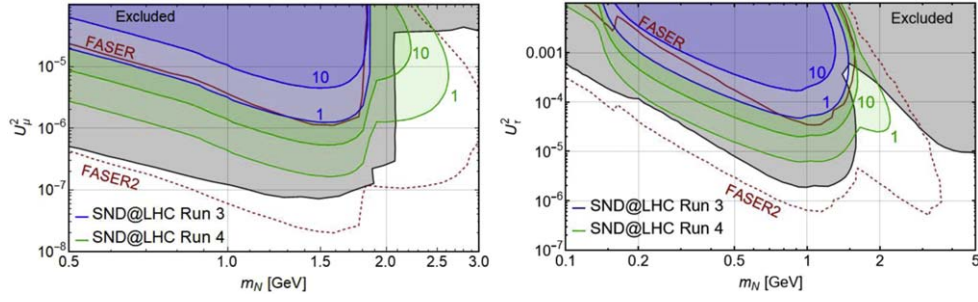
Figure 17. FASER and SND@LHC? reach for the HNL that mixes only with the muon neutrino \nu_\mu (left) and only with the tau neutrino \nu_\tau (right). The gray-shaded regions are excluded by current limits. Solid blue (green) contours correspond to 1 and 10 events in the (upgraded) SND@LHC target. FASER and FASER2 results are also reproduced. Figure is taken from [479].
