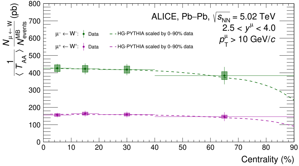
Figure 10. \langle T_{AA} \rangle -scaled yield of muons from W^- and W^+ decays in Pb-Pb collisions at \sqrt{s_{NN}} = 5.02 TeV for muons with p_T^{\mu} > 10 GeV/c and 2.5 < y_{\text{cms}}^{\mu} < 4.0 . The measured production is compared with HG-PYTHIA [74] calculations of the R_{AA} of hard scatterings scaled with the centrality-averaged production in 0–90% centrality, indicated as dashed lines. The horizontal bars correspond to the width of the centrality intervals, the vertical bars and boxes indicate the statistical and systematic uncertainties, respectively.
