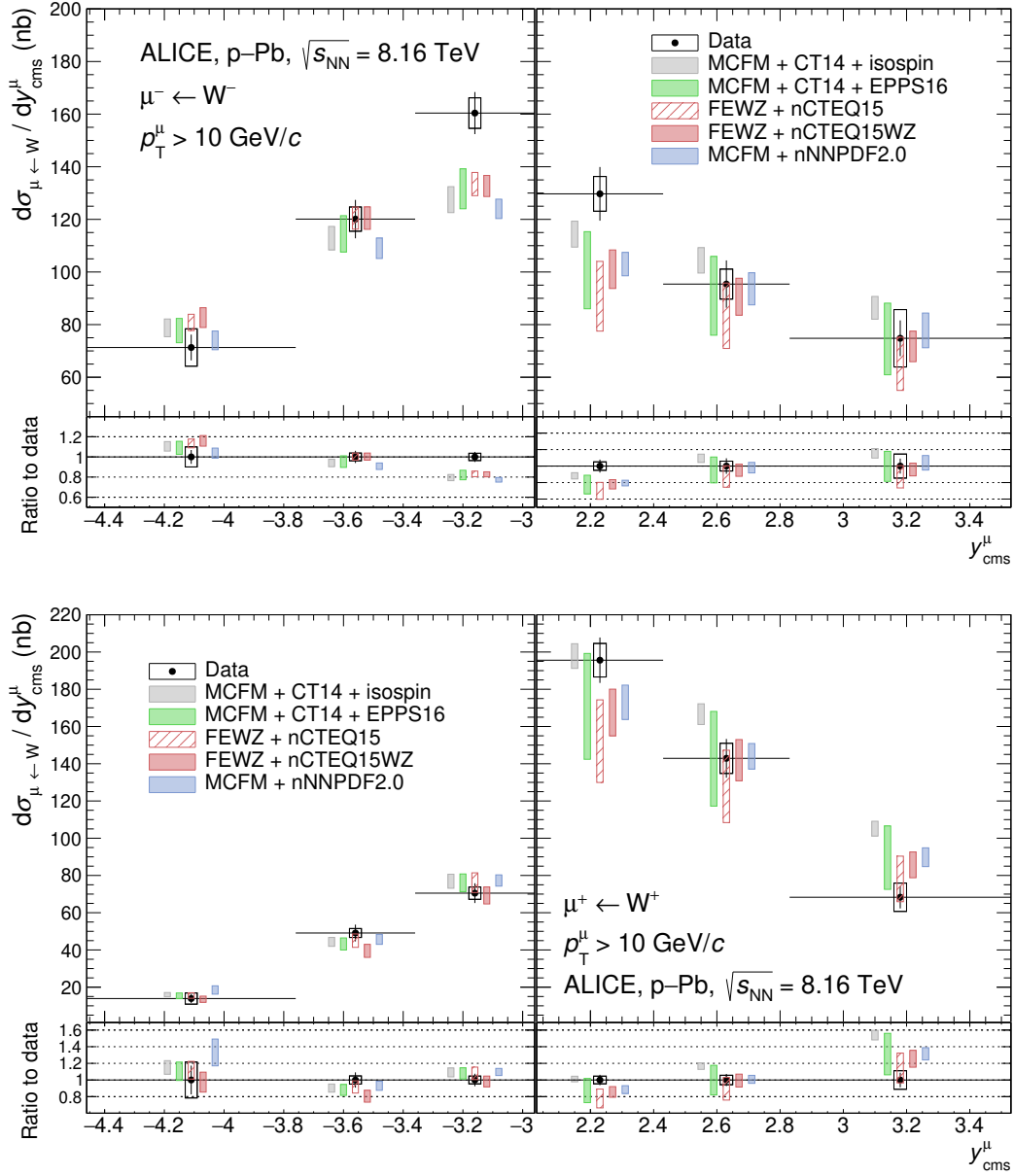
Figure 3. Production cross section of muons from W^- (top) and W^+ (bottom) decays as a function of rapidity for muons with p_T^{\mu} > 10 \text{ GeV}/c in p-Pb collisions at \sqrt{s_{\text{NN}}} = 8.16 \text{ TeV} . The measurements are compared with predictions from several nPDF sets, as well as with calculations based on the CT14 PDF set [67] without nuclear modifications of the PDF. All the calculations include the isospin effect. The bottom panels show the ratio of the calculations to the measured production cross section. The horizontal bars correspond to the width of the rapidity intervals. The vertical bars and boxes indicate the statistical and systematic uncertainties, respectively. The data points are placed at the centres of the rapidity intervals, while the theory predictions are horizontally shifted for better visibility.
