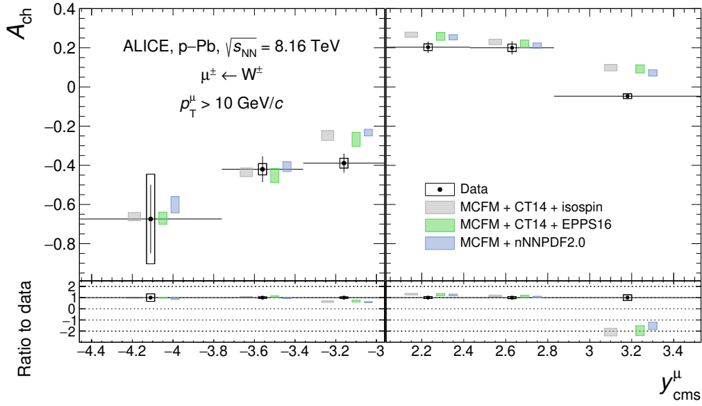
Figure 5. Lepton charge asymmetry for muons from W^{\pm} -boson decays with p_{\text{T}}^{\mu} > 10 GeV/ c in p-Pb collisions at \sqrt{s_{\text{NN}}} = 8.16 TeV. The measurements are compared with predictions from pQCD calculations with several nPDF sets as well as with calculations based on the CT14 PDF [67] without nuclear modifications. All the calculations include the isospin effect. The bottom panels show the ratio of the calculated to the measured asymmetry. The horizontal bars correspond to the width of the rapidity intervals. The vertical bars and boxes indicate the statistical and systematic uncertainties, respectively. The data points are placed at the centres of the rapidity intervals while the theory points are horizontally shifted for better visibility.
