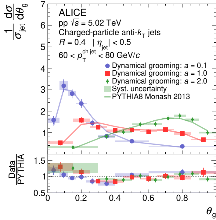
Figure 6. ALICE measurements of \theta_g distributions in pp collisions at \sqrt{s} = 5.02 \text{ TeV} with dynamical grooming [16] for three values of the grooming parameter a , compared with PYTHIA8 Monash 2013 [42, 43] calculations.
