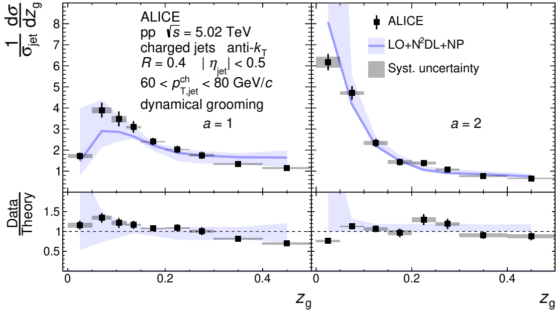
Figure 7. ALICE measurements of z_g distributions in pp collisions at \sqrt{s} = 5.02 \text{ TeV} with dynamical grooming for two values of the grooming parameter a , compared with pQCD calculations [16, 18].
