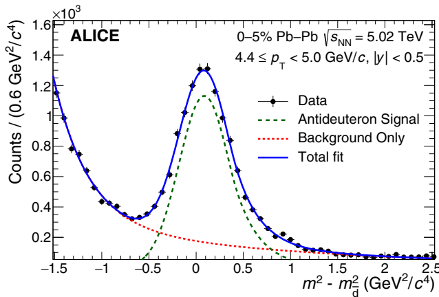
FIG. 2. Fit to the measured squared mass to extract the antideuteron signal in 4.4 < p_T < 5.0 GeV/c (left) and the antitreron signal in 2.0 < p_T < 2.4 GeV/c (right). The red dashed line shows the background, the solid blue line the combined fit to the data, and the green dashed line the signal only.
