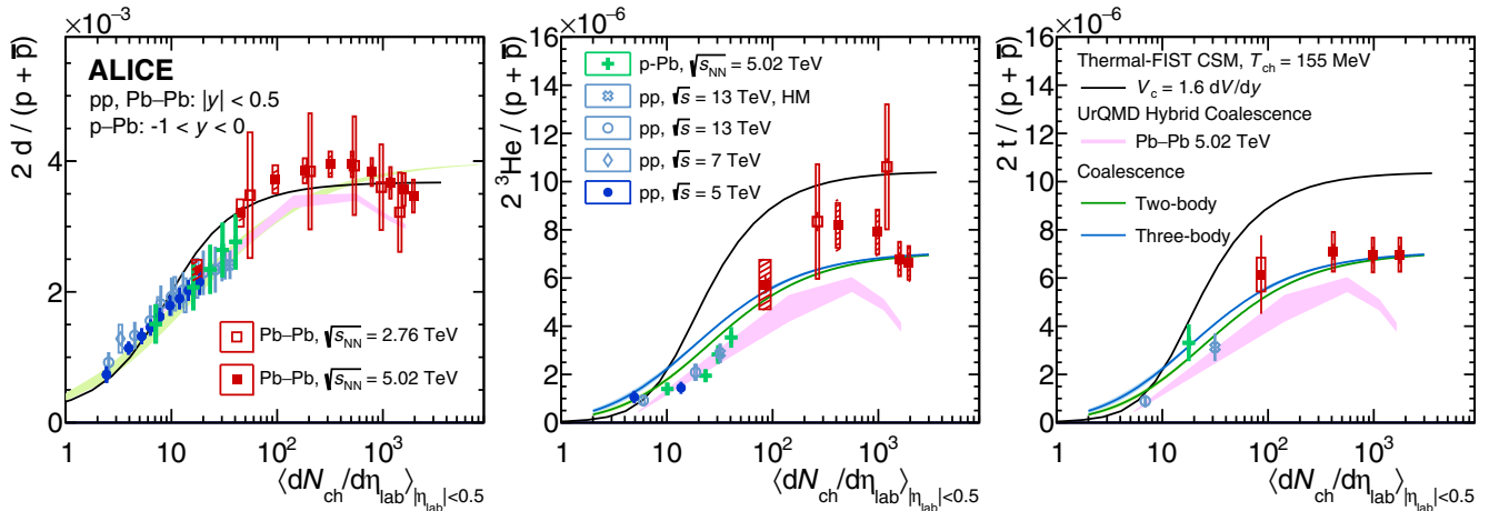
FIG. 7. Integrated deuteron (left), ^3\text{He} (middle), and triton yields (right) over proton yields as a function of charged-particle multiplicity \langle dN/d\eta_{ch} \rangle for pp, p–Pb, and Pb–Pb collisions measured by the ALICE Collaboration. The boxes represent the uncorrelated systematic uncertainties, while the vertical lines are the statistical ones. The shaded boxes represent the centrality-correlated uncertainties. In addition, the data are compared to the THERMAL-FIST CSM (canonical statistical model) at 155 MeV with a correlation volume of V_c = 1.6 dV/dy shown as a black line [58], the two coalescence approaches displayed in green (two-body coalescence) and in blue (three-body coalescence) [57], and URQMD hybrid coalescence shown as a purple line [86].
