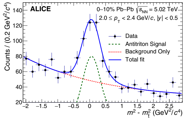
FIG. 2. Fit to the measured squared mass to extract the antideuteron signal in 4.4 < p_T < 5.0 GeV/c (left) and the antitreron signal in 2.0 < p_T < 2.4 GeV/c (right). The red dashed line shows the background, the solid blue line the combined fit to the data, and the green dashed line the signal only.
