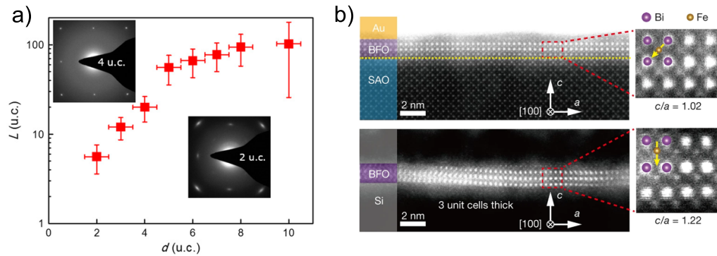
Figure 3. (a) Crystalline coherence length L as a function of thickness for \text{SrTiO}_3 suspended membranes. The insets are diffraction patterns obtained in TEM. From [57]. Reprinted with permission from AAAS. (b) Cross-sectional HAADF images of a 3-unit-cell-thick \text{BiFeO}_3 film before (top) and after (bottom) epitaxial liftoff. The insets show the transformation from rhombohedral to tetragonal symmetry and the corresponding polar displacement. Reproduced from [58], with permission from Springer Nature.
