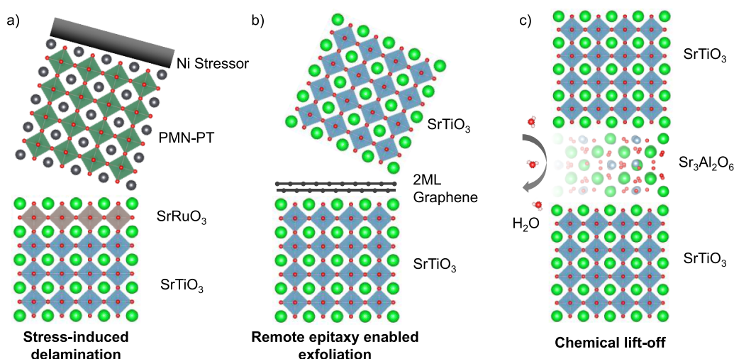
Figure 2. Representative methods developed recently to fabricate freestanding membranes of complex oxides, including: (a) mechanical release, via stress-induced breaking of weakly bonded interfaces; (b) exfoliation enabled via intercalated graphene; and (c) chemical etching of a sacrificial layer. (a,b) reproduced from [79], with permission from Springer Nature.
