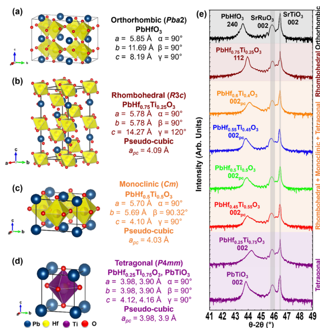
Figure 1. Crystal structure and lattice parameters for (a) the orthorhombic ( Pba2 ) antiferroelectric phase of \text{PbHfO}_3 , (b) the rhombohedral ( R3c ) ferroelectric phase of \text{PbHf}_{0.75}\text{Ti}_{0.25}\text{O}_3 , (c) the monoclinic ( Cm ) ferroelectric phase of \text{PbHf}_{0.5}\text{Ti}_{0.5}\text{O}_3 , and (d) the tetragonal ( P4mm ) ferroelectric phase of \text{PbHf}_{0.25}\text{Ti}_{0.75}\text{O}_3 and \text{PbTiO}_3 . (e) X-ray-diffraction measurements ( \theta – 2\theta line scan) for 200-nm-thick, (240_O) -oriented \text{PbHfO}_3 , 112_R -oriented \text{PbHf}_{0.75}\text{Ti}_{0.25}\text{O}_3 , and 002_{pc} -oriented \text{PbHf}_{1-x}\text{Ti}_x\text{O}_3 (with x = 0.4, 0.45, 0.5, 0.55, 0.75 , and 1) heterostructures grown on 40 nm \text{SrRuO}_3/\text{SrTiO}_3(001) substrates.
