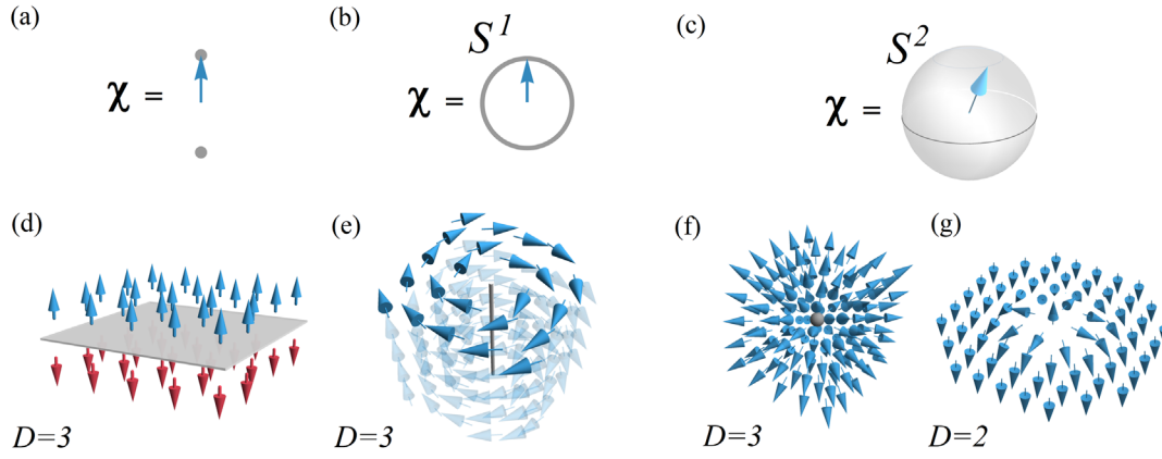
FIG. 2. Order-parameter spaces \mathcal{X} for (a) the Ising, (b) XY, and (c) Heisenberg models. The arrows indicate examples of orientations of the spin vector. The locus of all possible spin tip positions constitute the order-parameter space. The relevant topological defects in three dimensions for the Ising, XY-, and Heisenberg models are (d) domain walls (e) vortex lines, and (f) hedgehogs or Bloch points. The Heisenberg model also allows for various topological solitons in D = 1, 2 , and 3 dimensions. (g) Néel skyrmion, which is an example of such a soliton. This can be considered the stereographic projection of (f) taken from the south pole.
