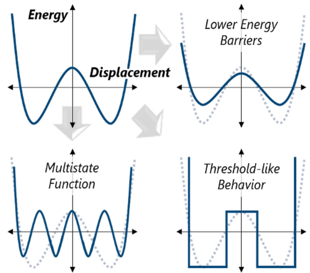
FIG. 41. Manipulating energy landscapes in ferroelectrics. The schematic illustration shows how the energy landscape can be manipulated to create tunable barrier heights, multistates, and thresholdlike behavior.
