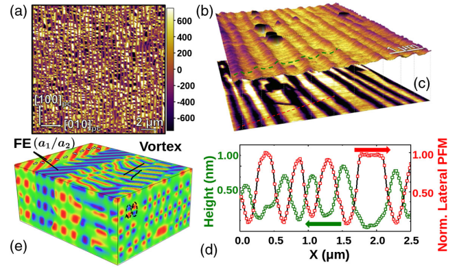
FIG. 22. (a) Lateral piezoresponse image for a \text{SrTiO}_3/\text{PbTiO}_3 superlattice with n=16 revealing striplike order in which alternating stripes exhibit high (checked white and black) and low or zero [brown (gray)] piezoresponse with a periodicity of \sim 300 nm along the [010]_{\text{pc}} . (b) Variations in the surface topography. (c) Changes in the lateral piezoresponse amplitude. (d) Line trace across the topography (green dashed line) and lateral piezoresponse images (red dashed line) revealing opposite and dramatic modulations in surface topography and lateral piezoresponse between the a_1/a_2 and vortex phases. These measurements in combination with RSM x-ray diffraction studies confirm that the vortex phase corresponds to protruding features in surface topography with low piezoresponse, while the a_1/a_2 phase is recessed in topography with large lateral piezoresponse. (e) 3D phase-field calculated image of the mixed vortex-ferroelectric a_1/a_2 phase ensemble. Adapted from Damodaran et al. , 2017a.
