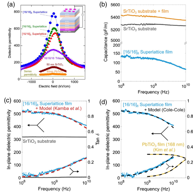
FIG. 46. (a) Dielectric permittivity as a function of electric field (applied voltage divided by the thickness of the sample) for \text{SrTiO}_3/\text{PbTiO}_3 superlattices with different periodicities. (b) Measured capacitance of coplanar wave guide (CPW) transmission lines on the superlattice (upper orange line) and the \text{SrTiO}_3 substrate (black middle line). Finite-element simulations and the measurements of the bare \text{SrTiO}_3 substrate are used to analyze and isolate the portion of the total capacitance that is related to the permittivity of the superlattice (bottom blue line). (c) The real part of the in-plane dielectric permittivity (left-hand y axis) and the loss tangent (right-hand y axis) are determined from the capacitance and conductance measurements via a mapping function obtained from 2D finite-element modeling of the CPW structures. (d) Cole-Cole model of the in-plane complex permittivity of the superlattice from 100 MHz to 10 GHz. From Das et al. , 2021.
