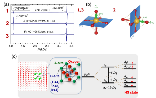
FIG. 47. (a) EPR spectrum from the [\text{Fe}^{3+} - \text{PbTiO}_3] . (b) Left image: schematic of the \text{Fe}^{3+} -doped \text{PbTiO}_3 [ \text{Fe}^{3+} - \text{PbTiO}_3 ] in the tetragonal perovskite structure, with the green up arrow indicating the polarization direction and the horizontal blue sheet the easy plane of the spins in \text{Fe}^{3+} . Right image: graphic showing that the easy plane of the spins rotates as the polarization direction is rotated by 90^\circ . (c) Schematic indicating what happens to the crystal-field splitting and spin-orbit coupling when an impurity is placed within a polar vortex (or skyrmion).
