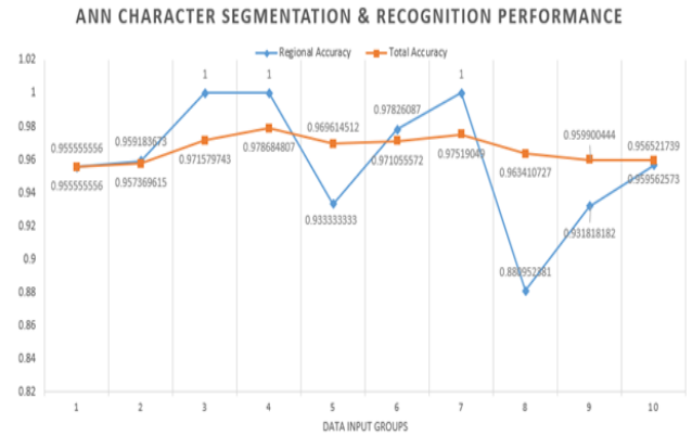
Figure 11: A Line Chart Representing Regional and Total Accuracy of ANN Character Segmentation and Recognition Algorithm
