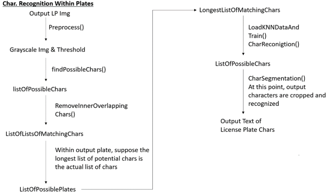
Figure 8: Basic Process of Character Segmentation and Recognition Program. The Two Processes Run Synchronized In Order To Improve Efficiency
