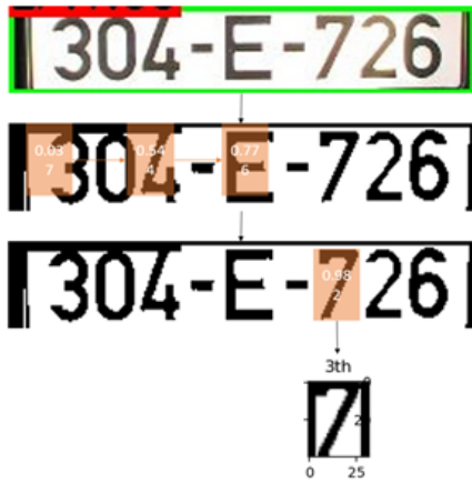
Figure 6: Character Segmentation Program Based on A Character Feature Detection Neural Network Can Evaluate Each Region's Score, thus Listing All Highly Potential Regions and Crop the Proper Characters
