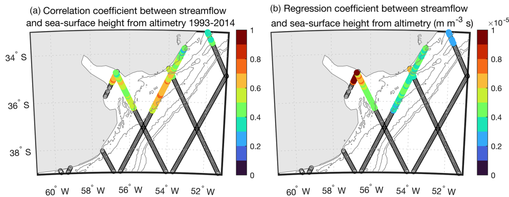
Figure 12. (a) Correlation coefficient and (b) regression coefficient ( \text{m m}^{-3} \text{ s} ) between annual streamflow in the Río de la Plata (Fig. 3) and sea surface height anomaly from along-track satellite altimetry data (Birol et al., 2017) during 1993–2014 over the study regions. Values are only shown where correlation coefficients are positive at the 95 % confidence level determined through bootstrapping. Contours identify the 20, 50, 100, 200, and 500 m isobaths.
