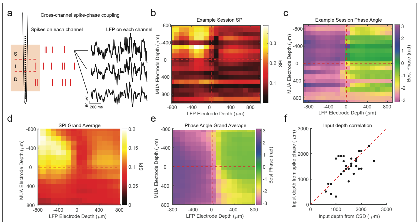
Figure 3. Cross-channel spike–local field potential (LFP) phase coupling reversal correlates with putative input layer. (a) Schematic displaying cross-channel phase coupling analysis. The spike times on each channel are compared against the phase of the LFP on each other channel, yielding a matrix of spike-phase coupling. (b) Example recording session cross-channel spike-phase index (SPI) values from marmoset MT. Red dashed lines indicate the estimated depth of the bottom of the input layer from current-source density (CSD) analysis. (c) Preferred phase angles for the cross-channel spike-phase relationships in b. Spikes across all channels preferred \pm\pi rad phase angles from LFP measure on superficial and input electrodes, but preferred 0 rad phase angles from LFP measured on deep phase angles. The LFP phase reversal aligns well to the estimate of the input layer from CSD analysis (red dashed line). (d) Grand average cross-channel SPI across all recording sessions in MT, V4, and PFC aligned to the putative input layer from CSD analysis ( N = 34 sessions). (e) Grand average of the preferred phase angle for the data in d. (f) Scatter plot shows a significant correlation between the depth of the bottom of the input layer estimated from CSD analysis (x-axis) and the depth of the phase reversal (y-axis; Pearson's r = 0.64 , p = 0.00005 ).
