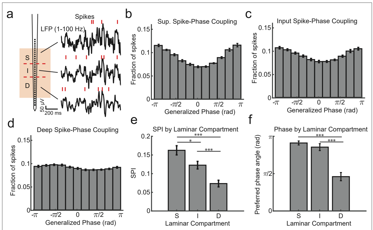
Figure 2. Within channel spike–local field potential (LFP) phase coupling strength and preferred phase angle varies across layers. (a) Spike–LFP phase coupling was measured by taking the phase of the LFP on a contact at the times when multi-unit spikes were detected on the same contact. (b) Spike–phase distribution for superficial contacts averaged across all recordings sessions ( N = 34 sessions across 4 monkeys; error bars denote standard error of the mean [SEM]). The spike–phase distribution was strongly peaked toward \pm\pi rad. (c, d) Same as b, but for contacts in the input and deep layers. (e) The average spike–phase index (SPI) was significantly weaker for input and deep layers relative to the superficial layer (0.16 vs. 0.12 and 0.07; p = 0.017 S. v. I. and p < 1 \times 10^{-7} S. v. D.; Wilcoxon signed-rank test; * p < 0.05 , *** p < 0.0001 ). (f) There was no difference in the preferred LFP phase angle between superficial and input layers, but a significant difference between these layers and deep layers ( -2.86 and -2.68 vs. -1.44 rad; F = 38.52 , p < 1 \times 10^{-7} and F = 21.15 , p = 0.00002 , respectively; Watson–Williams test).
