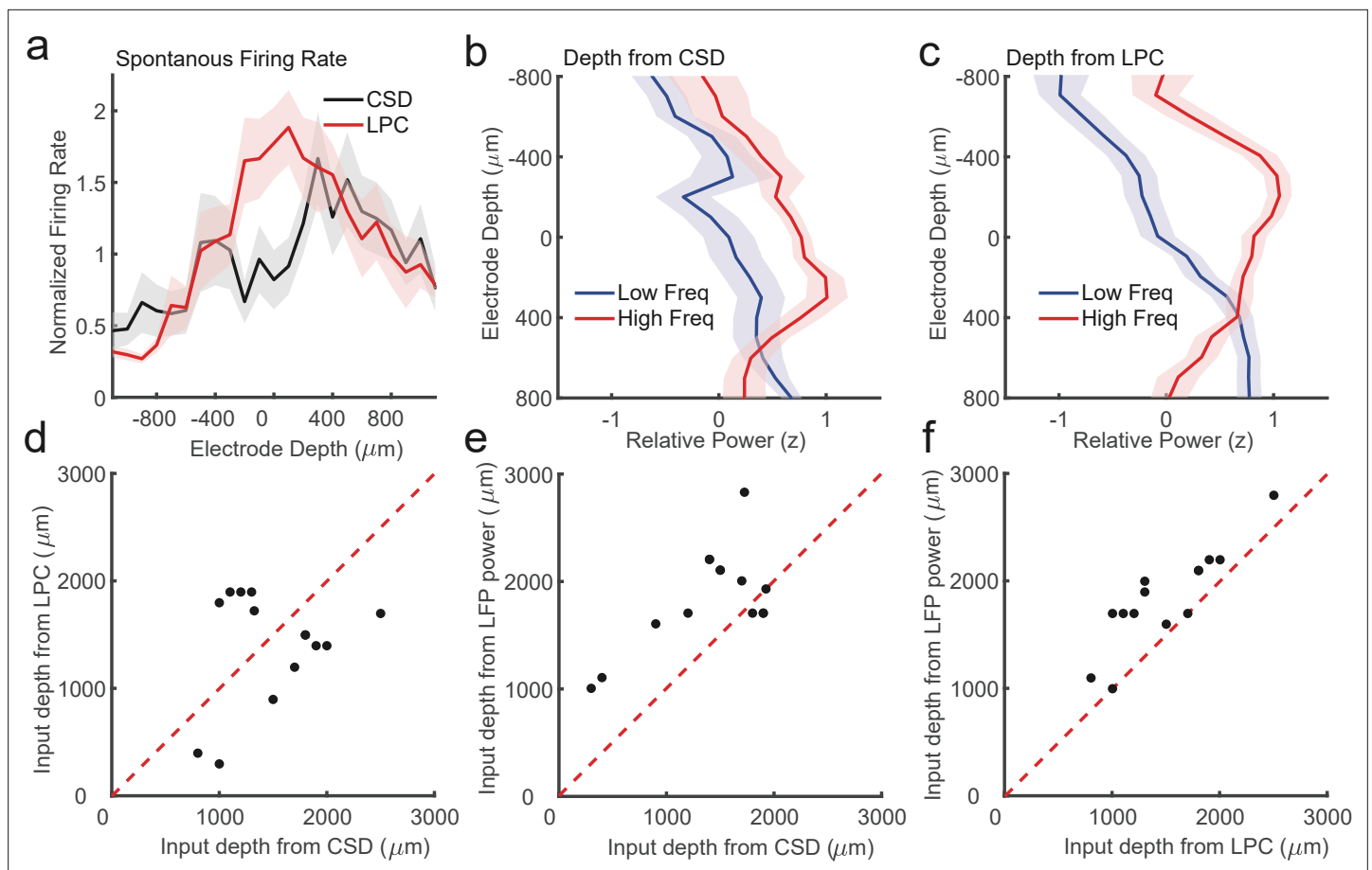
Figure 6. Laminar-phase coupling (LPC) pattern better replicates spike rate and local field potential (LFP) power dissociations than current-source density (CSD) when the two measures disagree. (a) Normalized spontaneous firing rates across sessions when CSD and LPC disagreed as a function of contact depth by more than 200 \mu\text{m} ( N = 14 ; shaded regions denote standard error of the mean [SEM]). LPC captures the expected higher spontaneous firing rates around the input layer. (b) Mean z-scored LFP power across sessions in lower frequencies (8–30 Hz, blue line) and higher frequencies (65–100 Hz, red line) as a function of electrode depth referenced to the CSD estimate for sessions. (c) Same as in a, but referenced to the depth estimate from the LPC phase reversal across sessions. The laminar power relationship is more pronounced when using the phase reversal instead of CSD estimate. (d) Scatter plot showing the disagreement in the depth of the input layer estimated from CSD (x-axis) and the depth from LPC (y-axis) in this subset of recording sessions. (e) Scatter plot showing the alignment of the CSD input depth (x-axis) crossover in LFP power (y-axis). (f) Same as e, but for LPC. The LPC depth measure was more correlated with the LFP power reversal than the CSD measure (Pearson's r = 0.65 vs. 0.87 CSD vs. LPC).
