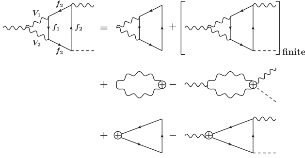
FIG. 2. Diagrammatic demonstration of VZH divergence separation. \square_{\text{finite}} denotes the finite integral after all subtractions have been applied.
