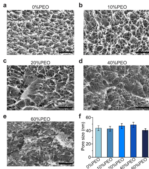
Fig. 3 The SEM cross-sectional images of B. mori silk films. (a) 0% PEO, (b) 10% PEO, (c) 20% PEO, (d) 40% PEO, and (e) 60% PEO. Scale bar, 500 nm. (f) Average pore diameters of porous silk. Error bars represent standard errors.
