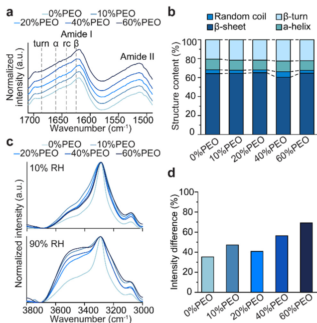
Fig. 4 (a) The FTIR spectra of silk amide I and II bands. (b) Secondary structure contents calculated from the deconvoluted amide I bands. (c) OH stretching bands of water of porous silk films at 10% RH and 90% RH. (d) Intensity difference of OH stretching bands as a function of PEO concentration.
