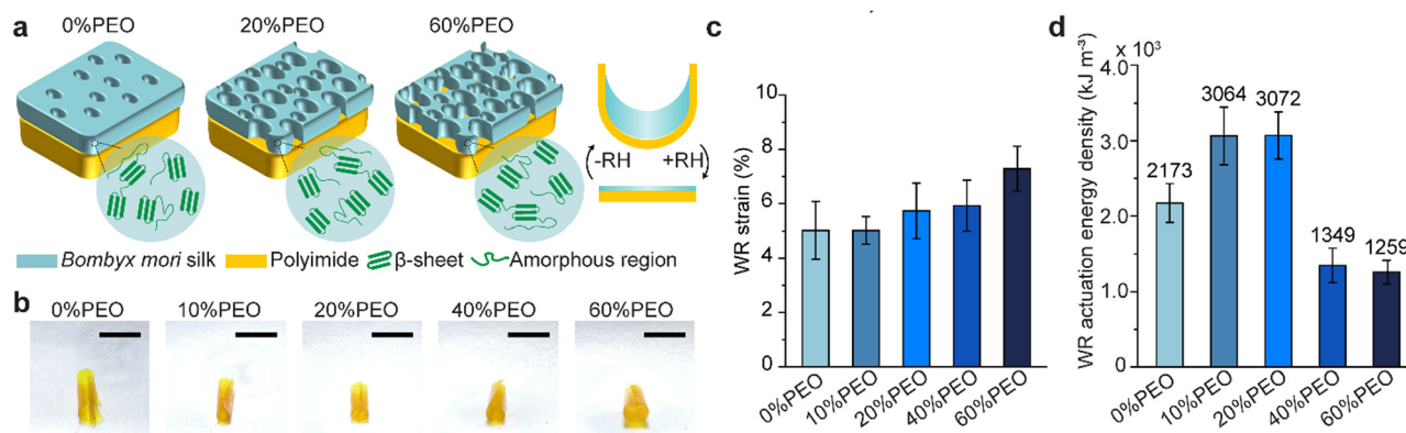
Fig. 1 (a) Schematic of silk/polyimide structures, where silk's porosity is varied by tuning the concentration of PEO. (b) Silk/polyimide bilayers bend at 10% RH. Scale bar, 3 mm. (c) WR strain of porous silk films. Error bars represent standard deviations determined from five different measurements ( n = 5 ). (d) Estimated WR actuation energy densities of porous silk. Error bars represent standard deviations determined from five different measurements ( n = 5 ).
