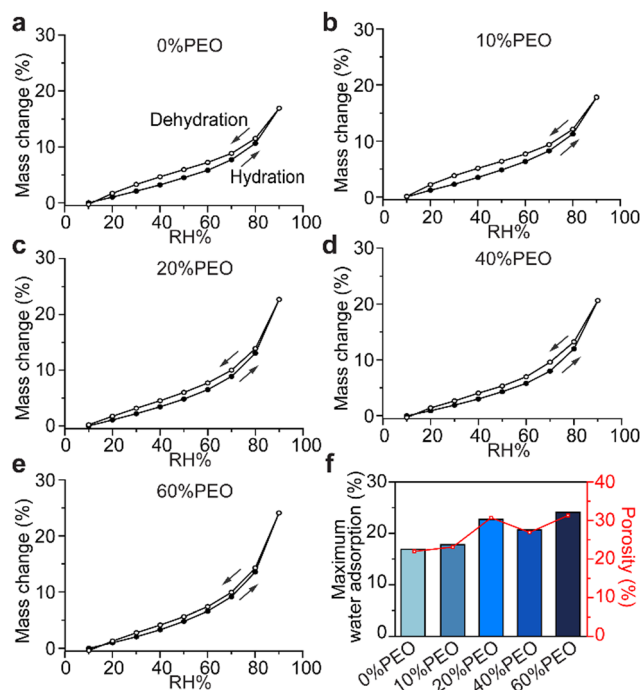
Fig. 2 (a–e) DVS water sorption isotherms of porous silk films. (f) Porous silk's maximum water adsorption and porosities.
