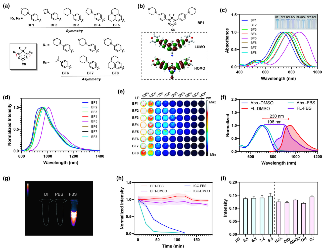
Figure 1. (a) Structures of BF 2 formazanate dyes BF1–BF8 in this study. (b) HOMOs and LUMOs calculated for BF1 . (c) The normalized absorbance spectra of BF1–BF8 (20 μM) solution in DMSO. Inset shows photos of the solutions. (d) The normalized fluorescence spectra of BF1–BF8 (20 μM) in DMSO. (e) False-colored images of BF1–BF8 at 50 μM collected through long-pass (LP) filters with cut-on wavelengths of 1000, 1050, 1100, 1150, 1200, 1250, 1300, 1350, and 1400 nm illumination was at 808 nm laser (45 mW cm -2 , 250 ms exposure). (f) Stokes shift of BF1 with a concentration of 10 μM in DMSO and FBS. (g) NIR-II fluorescence images of BF1 (10 μM) in deionized water (DI), PBS buffer, and FBS. (h) Stability of BF1 and ICG (10 μM) under 808 nm light radiation within 180 minutes in FBS and DMSO. (i) Fluorescent stability of BF1 (10 μM) in PBS (1% FBS) buffer with different pH and ROS species.
