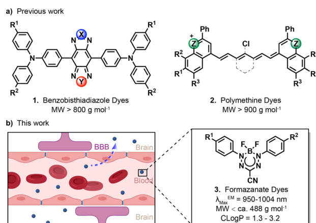
Scheme 1. Small-molecule scaffolds with NIR-II fluorescence. (a) Previous molecules which possess NIR-II fluorescence. (b) The schematic diagram of BF 2 formazanate dyes penetrating the BBB from the circulation.
