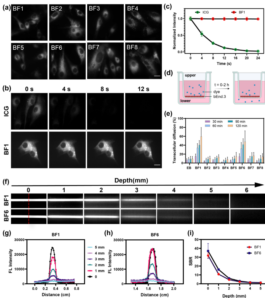
Figure 2. (a) Fluorescence imaging of BF1–BF8 in U-87 MG cells. All cell imaging experiments were performed using an NIR-II microscope with a 663 nm excitation laser (200 W cm −2 , exposure 10 ms) and 950 ± 50 nm emission filter. Scale bar is 10 \mu m. (b) Fluorescence imaging of ICG and BF1 in U-87 MG cells at 0, 4, 8, 12 s under laser irradiation. Scale bar is 10 \mu m. (c) Cellular photostability curves of ICG and BF1 within 25 seconds. (d) Schematic diagram of in vitro BBB model used in this study. (e) The relative transcellular diffusion amount of BF1–BF8 and EB in vitro within 2 hours. (f) Fluorescence images (excitation 808 nm, LP 1000 nm) of the capillary tube filled with BF1 and BF6 at depths of 0–6 mm in 1% Intralipid mimic tissue. (g, h) The cross-sectional fluorescence intensity profiles of BF1 and BF6 along the red dash line in (f) at different tissue depths. (i) The signal-background ratio (SBR) curves of BF1 and BF6 in 1% Intralipid®.
