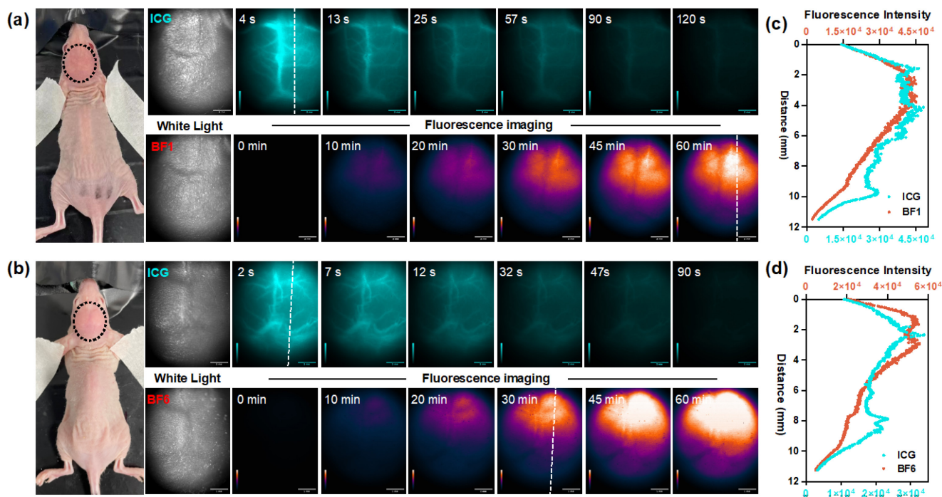
Figure 4. (a) White light and noninvasively in vivo NIR-II fluorescence imaging of mouse brains bearing primary glioma tumor after treating ICG and BF1 (200 \mu M, 200 \mu L, tail vein injection) at six time points (4, 13, 25, 57, 90, 120 s for ICG; 0, 10, 20, 30, 45, 60 min for BF1 ). (b) White light and noninvasively in vivo NIR-II fluorescence imaging of mouse brains bearing primary glioma tumor after treating ICG and BF6 (200 \mu M, 200 \mu L, tail vein injection) at six time points (2, 7, 12, 32, 47, 90 s for ICG; 0, 10, 20, 30, 45, 60 min for BF6 ), respectively. The laser power was 70 mW cm -2 , 808 nm laser, 1000 nm LP filter; (c, d) Cross-sectional fluorescence intensity profile along the white dash lines in (a) and (b) collected by 1000 nm long-pass filter.
