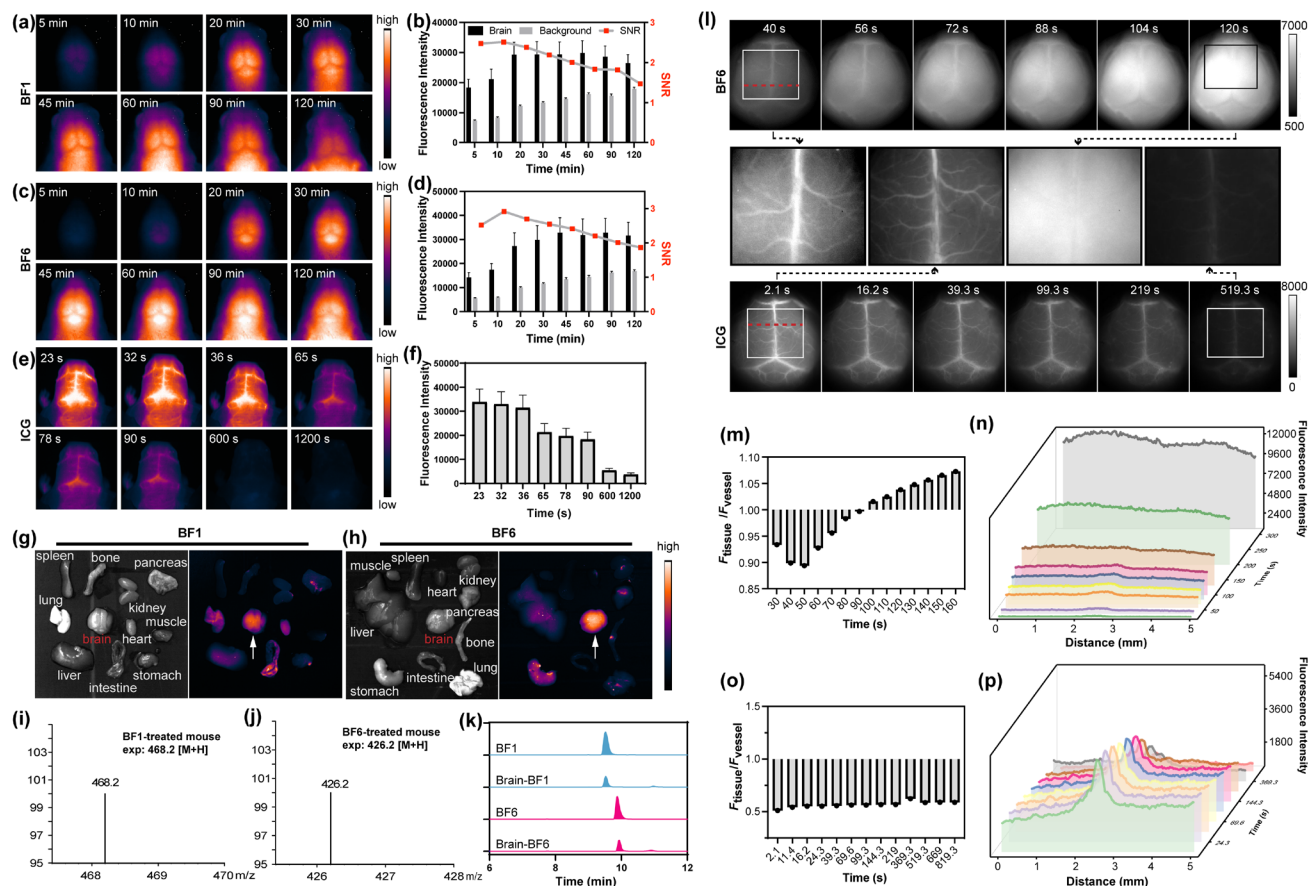
Figure 3. (a) In vivo NIR-II fluorescence imaging of cerebral tissue of mice injected with BF1 (200 \mu L, 200 \mu M, tail vein injection) at time intervals from 5 to 120 min. (70 mW \text{cm}^{-2} , 808 nm laser, 1000 nm LP filter). (b) Time-dependent signal-to-noise ratio (SNR) changes determined by the NIR-II fluorescence imaging of BF1 -treated mice. (c) In vivo NIR-II fluorescence imaging of cerebral tissue of mice injected with BF6 as described in (a). (d) SNR changes of BF6 -treated mice. (e) In vivo NIR-II fluorescence imaging of cerebral tissue from nude mice injected with ICG (200 \mu L, 200 \mu M) at certain time intervals from 5 s to 1200 s. (f) The fluorescence intensity changes of the brain at designated time points. (g, h) The fluorescence images of the heart, lung, kidney, spleen, liver, brain, intestine, stomach, bone, muscle, and pancreas at 2 hour after the injection of BF1 and BF6 . (i, j) Mass spectra from extracted brain tissue of mice after intravenous injection of BF1 and BF6 for 1 hour. (k) HPLC spectra of BF1 , BF6 standards and responding brain homogenate of mice treated with BF1 and BF6 . (l) In vivo NIR-II fluorescence imaging change of brain vessels and tissue at different time points after intravenous injection of BF6 and ICG. (m) Fluorescence ratio changes of brain tissue and vessel after intravenous injection of BF6 in (l) at different time points. (n) Cross sectional fluorescence intensity profile along the red dash line in (l) collected by a 1000 nm long-pass filter at designated time points after intravenous injection of BF6 . (o) Fluorescence ratio changes of brain tissue and vessel after intravenous injection of ICG in (l) at different time points. (p) Cross sectional fluorescence intensity profile along the red line in (l) collected by a 1000 nm long-pass filter at designated time points after intravenous injection of ICG.
