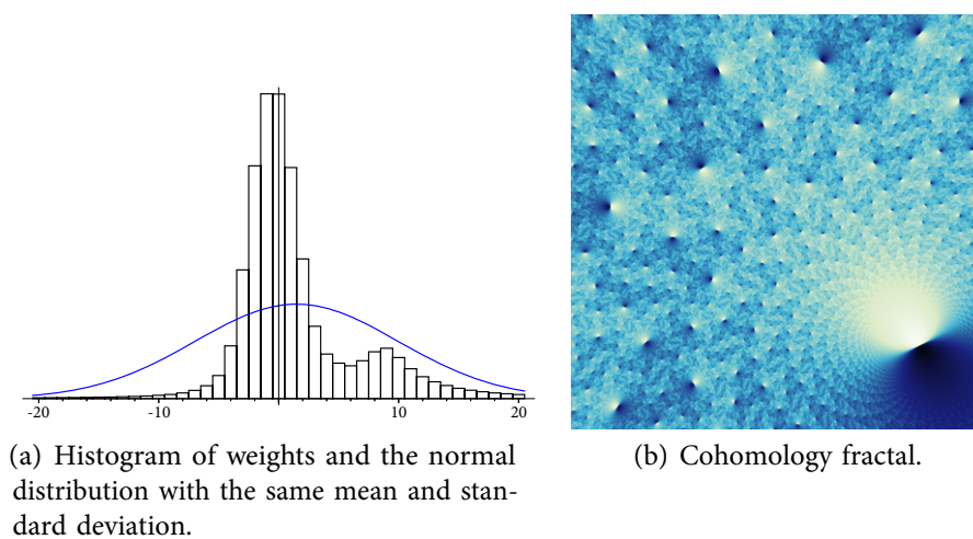
Figure 22. Statistics for a cohomology fractal of s789 for a class not vanishing on cusp.
