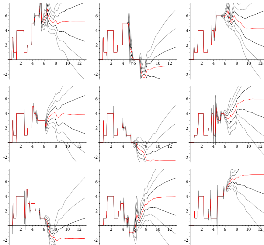
Figure 19. The graph of the average value of the cohomology fractal for m122(4, -1) for various square regions U with field of view 0.1^\circ . Thus, these are the same size as the pixels of Figure 18. These are each computed by taking 1000 \times 1000 samples. We also show the envelopes of 0.5, 1.0 and 1.5 standard deviations.
