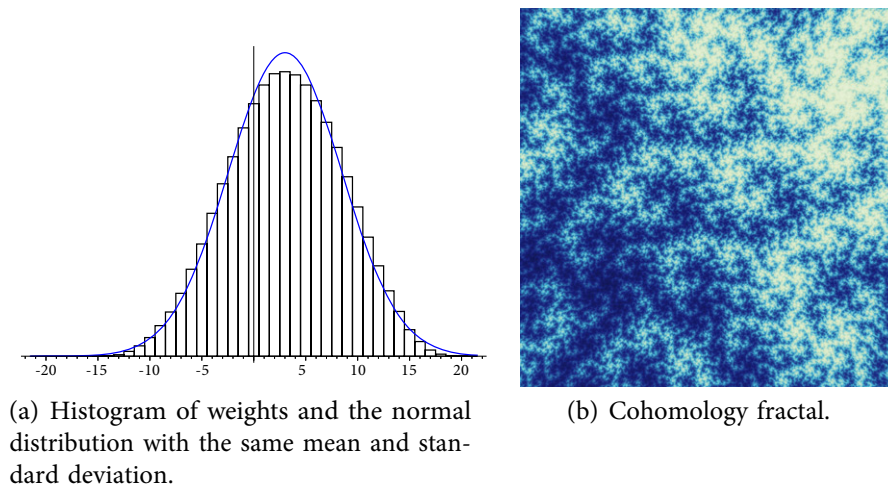
Figure 20. Statistics for a cohomology fractal of m122(4, -1) for a square region with field of view 20^\circ and R = e^2 .
