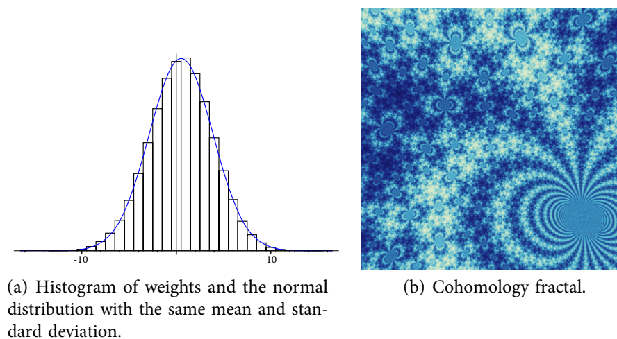
Figure 21. Statistics for a cohomology fractal of s789 for a class vanishing on cusp.
