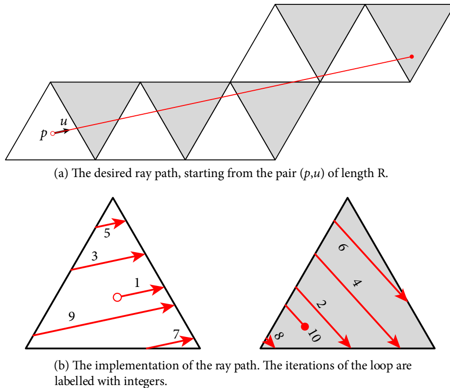
Figure 7. A toy example of developing a ray through a tiling of a euclidean torus. Note that the geodesic segments passing through a tile are parallel; this is only because the geometry is euclidean. In a hyperbolic tiling the segments are much less ordered.
