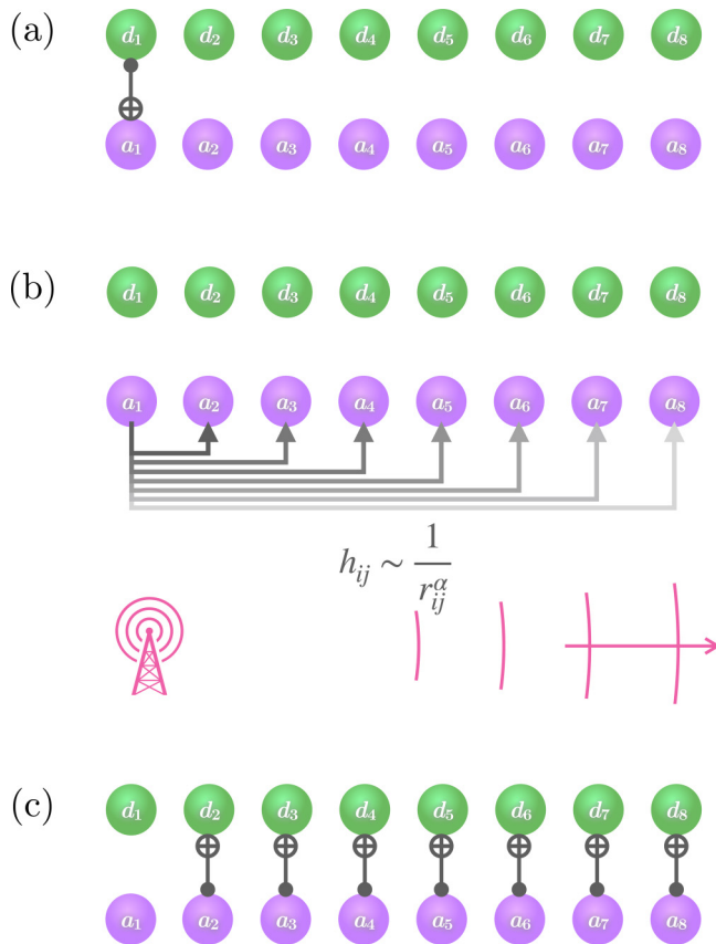
FIG. 1. A protocol for a fast unbounded quantum fanout gate using long-range interactions, depicted here for a 1D lattice. The layout consists of a chain of data qubits, along with their adjacent ancillary qubits that are initialized to |0\rangle . (a) The first step is a local controlled-NOT (CNOT) gate from |d_1\rangle to |a_1\rangle . (b) The application of the long-range “broadcast” from |a_1\rangle to the rest of the ancillary qubits |a_i\rangle creates a GHZ-like state in Eq. (1) for the ancillary qubits together with the first data qubit. (c) We apply CNOT gates from ancillary qubit |a_i\rangle to the data qubit |d_i\rangle , which can be done in parallel. After this step, we reverse process (b) and process (a) to return the ancillary qubits to |0\rangle (not redrawn here).
