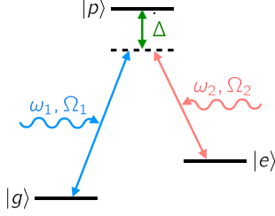
FIG. 5. Coupling scheme for two-photon Rabi oscillations in a \Lambda configuration, for states |g\rangle , |e\rangle , and |p\rangle . In the setup considered here, the two driving frequencies are assumed to differ by the qubit frequency: \hbar(\omega_1 - \omega_2) = E_e - E_g . The figure also shows the associated Rabi angular frequencies \Omega_1 and \Omega_2 , and the detuning \Delta .
