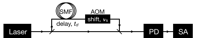
FIG. 1. Self-heterodyne setup. The laser signal is split equally between two paths. One path passes through a single-mode fiber (SMF), where it is delayed by time t_d . It then passes through an acousto-optic modulator (AOM), where its frequency is shifted by \nu_s . The interfering signals are combined and measured by a photodiode (PD), and finally processed through a spectrum analyzer (SA).
