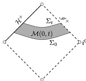
Figure 6. Penrose diagram of a black hole solution.
