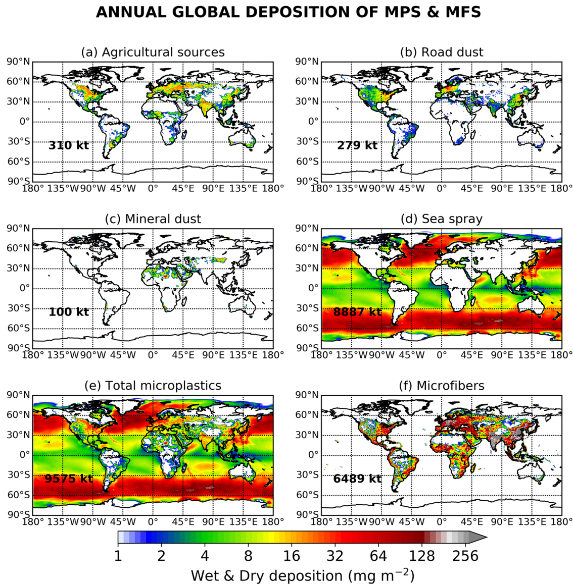
Fig. 5. Annual global deposition of MPs emitted from agriculture, with road and mineral dust and with sea spray. The annual global deposition of MFs from the global population is also given in the lower right panel.
