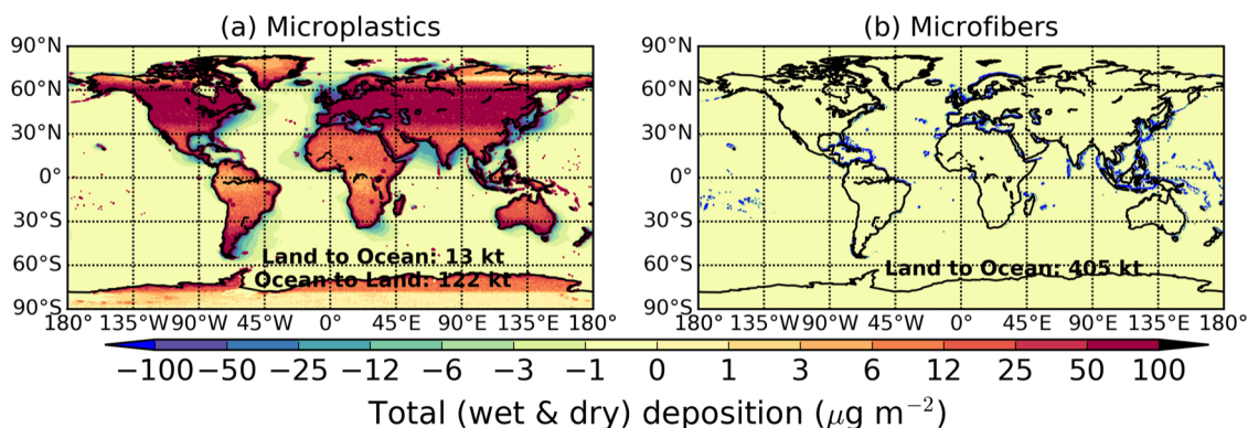
Fig. 7. (a) MPs emitted from the land that were deposited over the ocean annually and vice versa (ocean to land). (b) MFs emitted from global population that were deposited in the ocean.
