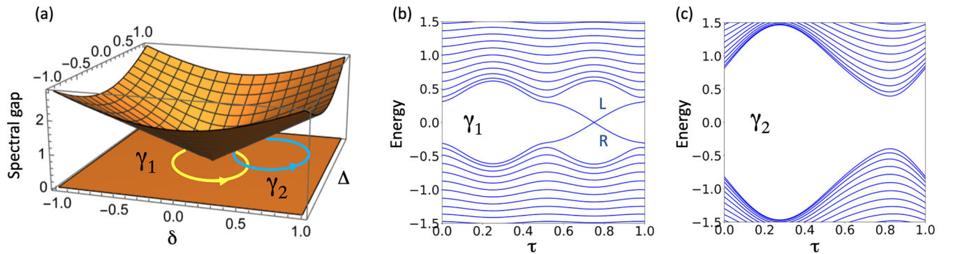
FIG. 2. (a) Spectral gap of the Hamiltonian (2) as a function of the parameters (\delta, \Delta) , together with two adiabatic cycles, of which \gamma_1 = [\delta = 0.3 \sin(2\pi\tau), \Delta = -0.3 \cos(2\pi\tau)] circles and \gamma_2 = [\delta = 0.4 + 0.3 \sin(2\pi\tau), \Delta = 0.4 - 0.3 \cos(2\pi\tau)] does not circle the gap singularity at \delta = \Delta = 0 . (b),(c) The energy spectrum of the Hamiltonian (2) as a function of the adiabatic parameter \tau for \gamma_1 and \gamma_2 , respectively. Both spectra are generated with chains of 20 sites. Two chiral modes located at opposite left (L) and right (R) ends of the chain are visible in panel (b). These chiral modes are absent for the adiabatic cycle \gamma_2 .
