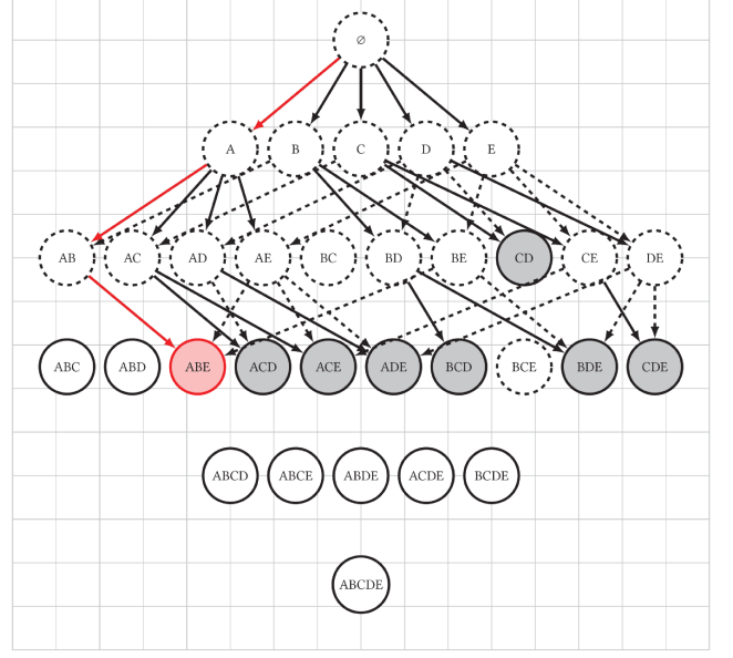
Figure 3: DAG representation.
