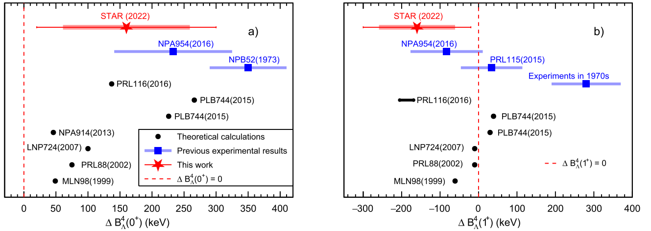
Fig. 5. The \Lambda binding-energy differences between {}^4_\Lambda\text{H} and {}^4_\Lambda\text{He} in ground states (a) and in excited states (b) compared with theoretical model calculations (black solid circles and a short black line) and previous measurements (blue solid squares). Solid error bars show statistical uncertainties and boxes show the systematic uncertainties. Red dashed vertical lines are drawn at \Delta B_\Lambda^4(0^+ \text{ or } 1^+) = 0 .
