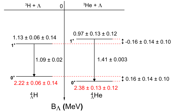
Fig. 4. Energy level schemes of {}^4_\Lambda\text{H} and {}^4_\Lambda\text{He} in terms of \Lambda binding energies. The ground-state binding energies are from this analysis. The values for excited states are obtained from the \gamma -ray transition energies measured in Refs. [11,38].
