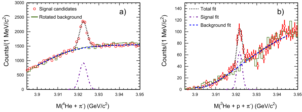
Fig. 2. Invariant-mass distributions for {}^4_\Lambda\text{H} (a) and {}^4_\Lambda\text{He} (b) reconstructed with KFPARTICLE and TMVA-BDT. The green histograms represent the rotated backgrounds. The blue dashed curves represent the background fits and are obtained by fitting the invariant-mass distributions outside of the signal regions with double-exponential functions. The black dashed curves are obtained by fitting these distributions across the full range of invariant mass with the background fit result and a Gaussian function. The violet dashed curves represent the signal Gaussian functions.
