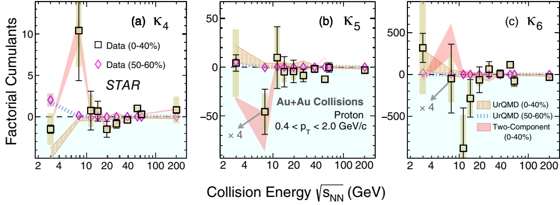
FIG. 2. \kappa_4 (a), \kappa_5 (b), \kappa_6 (c) of proton distribution in Au + Au collisions from 3 to 200 GeV. The results are shown for 0%–40% (squares) and 50%–60% (diamonds) centralities. The bars and bands on the data points represent the statistical and systematic uncertainties, respectively. The two-component model (0%–40%) and UrQMD model (0%–40% and 50%–60%) calculations are shown as red, brown bands, and blue dashed lines, respectively. The two-component model (with binomial and Poissonian distributions as constituent components) requires \kappa_n up to the fourth order as inputs to predict \kappa_5 and \kappa_6 . Uncertainties are statistical for the model calculations. The \kappa_5 and \kappa_6 data at 7.7 GeV (0%–40%) are scaled down by a factor of 4 for clarity of presentation.
