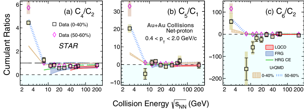
FIG. 3. C_4/C_2 (a), C_5/C_1 (b), and C_6/C_2 (c) of the net-proton distribution in Au + Au collisions from 3 to 200 GeV. The results are shown for 0%–40% (squares) and 50%–60% (diamonds) centralities. The bars and bands on the data points represent the statistical and systematic uncertainties, respectively. LQCD (39–200 GeV) [26], FRG (11.5–200 GeV) [27], UrQMD (0%–40%, 50%–60%), and HRG model calculations (7.7–200 GeV) with canonical ensemble [52] (HRG CE) are shown as red, gray, brown bands, blue and green dashed lines, respectively.
