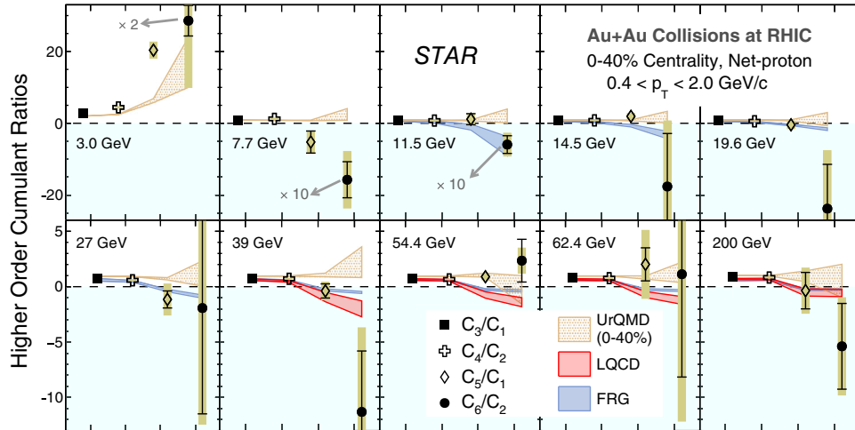
FIG. 4. C_3/C_1 (filled square), C_4/C_2 (open cross), C_5/C_1 (open diamond), and C_6/C_2 (filled circle) of net-proton distributions in 0%–40% Au + Au collisions from 3 to 200 GeV. The bars and bands on the data points represent the statistical and systematic uncertainties, respectively. LQCD (39–200 GeV) [26], FRG (11.5–200 GeV) [27] and UrQMD calculations (0%–40% centrality) are shown as red, blue, and brown bands, respectively. The C_6/C_2 data at 3 GeV (7.7 and 11.5 GeV) are scaled down by a factor of 2 (10) for clarity of presentation.
