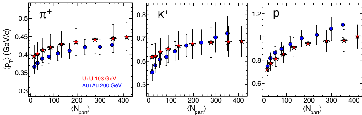
FIG. 5. \langle p_T \rangle of \pi^+ , K^+ , and p as a function of \langle N_{part} \rangle at midrapidity ( |y| < 0.1 ) for U+U collisions at \sqrt{s_{NN}} = 193 GeV. The results are compared with Au+Au collisions at \sqrt{s_{NN}} = 200 GeV [58]. The uncertainties represent the total systematic and statistical uncertainties added in quadrature, and are dominated by systematic uncertainties.
