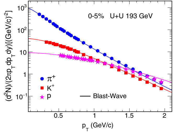
FIG. 9. Simultaneous blast-wave fit to the \pi^\pm , K^\pm , p ( \bar{p} ) p_T spectra in U+U collisions at \sqrt{s_{NN}} = 193 GeV in 0–5% centrality class within |y| < 0.1 . For clarity only distributions for positively charged particles are shown. The uncertainties represent the total systematic and statistical uncertainties added in quadrature.
