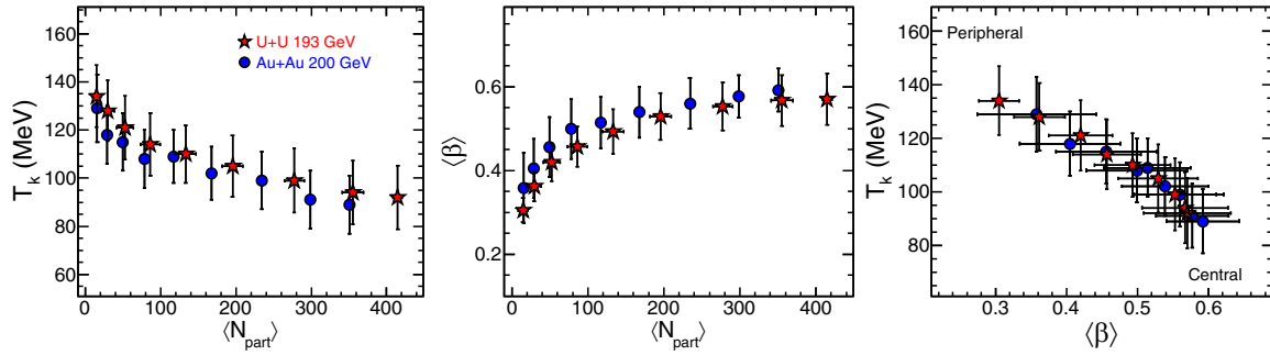
FIG. 10. Left panel: T_k as a function of \langle N_{\text{part}} \rangle . Middle panel: \langle\beta\rangle as a function of \langle N_{\text{part}} \rangle . Right panel: variation of T_k with \langle\beta\rangle . The midrapidity ( |y| < 0.1 ) results from U+U collisions at \sqrt{s_{NN}} = 193 GeV are compared with Au+Au collisions at \sqrt{s_{NN}} = 200 GeV [58]. The uncertainties represent the total systematic and statistical uncertainties added in quadrature, dominated by systematic uncertainties.
