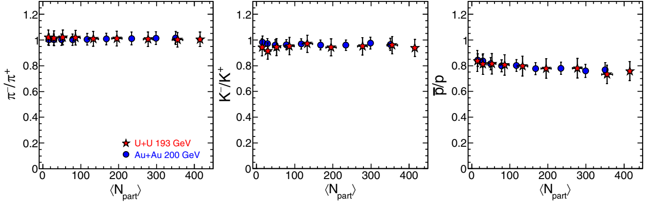
FIG. 7. \pi^-/\pi^+ , K^-/K^+ , and \bar{p}/p ratios at midrapidity ( |y| < 0.1 ) as a function of \langle N_{\text{part}} \rangle in U+U collisions at \sqrt{s_{NN}} = 193 GeV. The results are compared with Au+Au collisions at \sqrt{s_{NN}} = 200 GeV [58]. The uncertainties represent total systematic and statistical uncertainties added in quadrature, dominated by systematic uncertainties.
