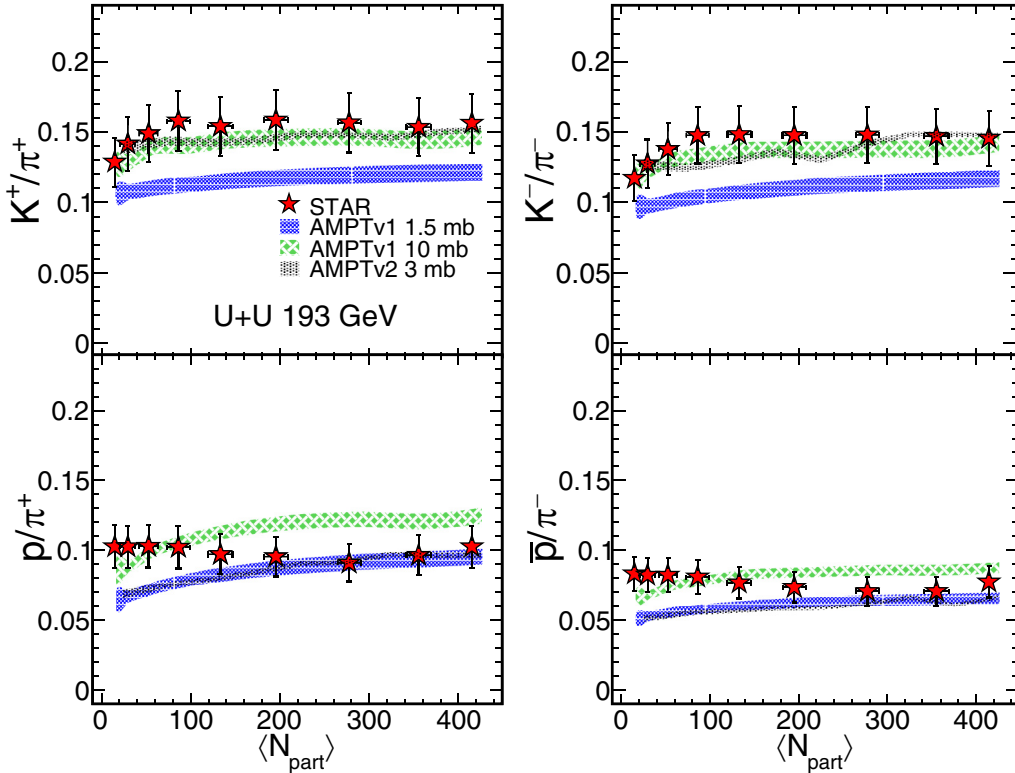
FIG. 14. K^+/\pi^+ , K^-/\pi^- , p/\pi^+ , and \bar{p}/\pi^- particle yield ratios at midrapidity ( |y| < 0.1 ) as a function of \langle N_{\text{part}} \rangle obtained for three calculations of AMPT data (AMPTv1 1.5 mb, AMPTv2 3 mb, and AMPTv1 10 mb) are shown along with the STAR results obtained in U+U collisions at \sqrt{s_{NN}} = 193 GeV. The width of the bands corresponds to the statistical uncertainty associated with the calculation using the AMPT model.
