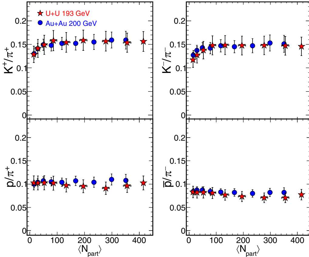
FIG. 8. K^+/\pi^+ , K^-/\pi^- , p/\pi^+ , and \bar{p}/\pi^- particle yield ratios at midrapidity ( |y| < 0.1 ) as a function of \langle N_{\text{part}} \rangle in U+U collisions at \sqrt{s_{NN}} = 193 GeV. The results are compared with Au+Au collisions at \sqrt{s_{NN}} = 200 GeV [58]. The uncertainties represent the total systematic and statistical uncertainties added in quadrature, dominated by systematic uncertainties.
