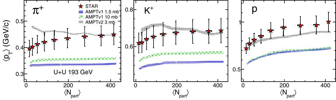
FIG. 11. \langle p_T \rangle of \pi^+ , K^+ , and p at midrapidity ( |y| < 0.1 ) as a function of \langle N_{\text{part}} \rangle obtained for the three sets of AMPT calculated data (AMPTv1 1.5 mb, AMPTv2 3 mb, and AMPTv1 10 mb) are shown along with the STAR results obtained in U+U collisions at \sqrt{s_{NN}} = 193 GeV. The width of the bands corresponds to the statistical uncertainty associated with the calculation using the AMPT model.
