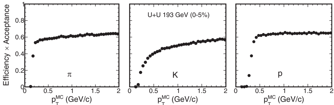
FIG. 3. Tracking efficiency \times acceptance as function of p_T^{\text{MC}} for reconstructed pions (left), kaons (middle), and protons (right) obtained from embedding in U+U collisions at \sqrt{s_{NN}} = 193 GeV. The errors are statistical only and within symbol size.
