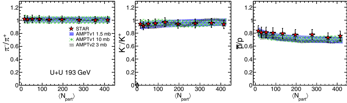
FIG. 13. \pi^-/\pi^+ , K^-/K^+ and \bar{p}/p particle yield ratios at midrapidity ( |y| < 0.1 ) as a function of \langle N_{\text{part}} \rangle obtained for three calculations of AMPT data (AMPTv1 1.5 mb, AMPTv2 3 mb, and AMPTv1 10 mb) are shown along with the STAR results obtained in U+U collisions at \sqrt{s_{NN}} = 193 GeV. The width of the bands corresponds to the statistical uncertainty associated with the calculation using the AMPT model.
