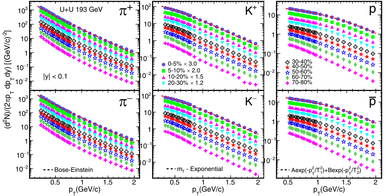
FIG. 4. p_T spectra of \pi^\pm , K^\pm , p ( \bar{p} ) measured at midrapidity ( |y| < 0.1 ) in U+U collisions at \sqrt{s_{NN}} = 193 GeV in STAR. Spectra are plotted for nine different centrality classes and some of them are scaled for clarity. The p_T spectra are fitted with Bose-Einstein function for pions, m_T exponential for kaons, and double exponential for (anti)protons, shown for 0–5% centrality classes in the figure. The uncertainties represent total systematic and statistical uncertainties added in quadrature and are mostly dominated by systematic errors.
