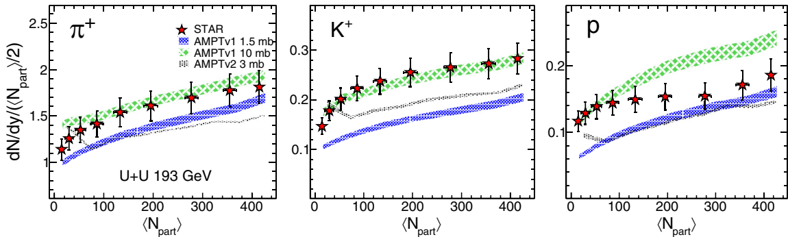
FIG. 12. dN/dy for \pi^+ , K^+ , and p scaled by \langle N_{\text{part}} \rangle / 2 at midrapidity ( |y| < 0.1 ) as a function of \langle N_{\text{part}} \rangle obtained for three calculations of AMPT data (AMPTv1 1.5 mb, AMPTv2 3 mb, and AMPTv1 10 mb) are shown along with the STAR results obtained in U+U collisions at \sqrt{s_{NN}} = 193 GeV. The width of the bands corresponds to the statistical uncertainty associated with the calculation using the AMPT model.
