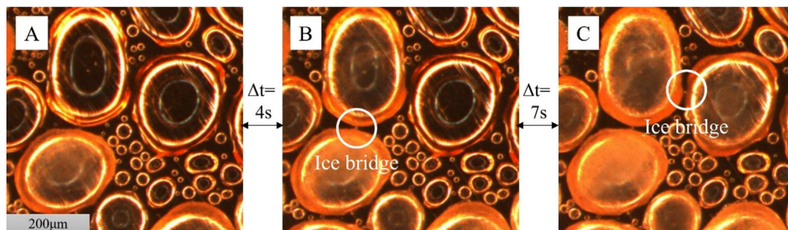
FIG. 3. Droplets freezing on the plain surface. (a) A droplet freezing before bridging to its neighbor. (b) The frozen droplet bridging to its neighbor causing it to freeze. (c) The newly frozen droplet bridging to its neighbor causing it to freeze. Multimedia view: https://doi.org/10.1063/5.0105412.1
