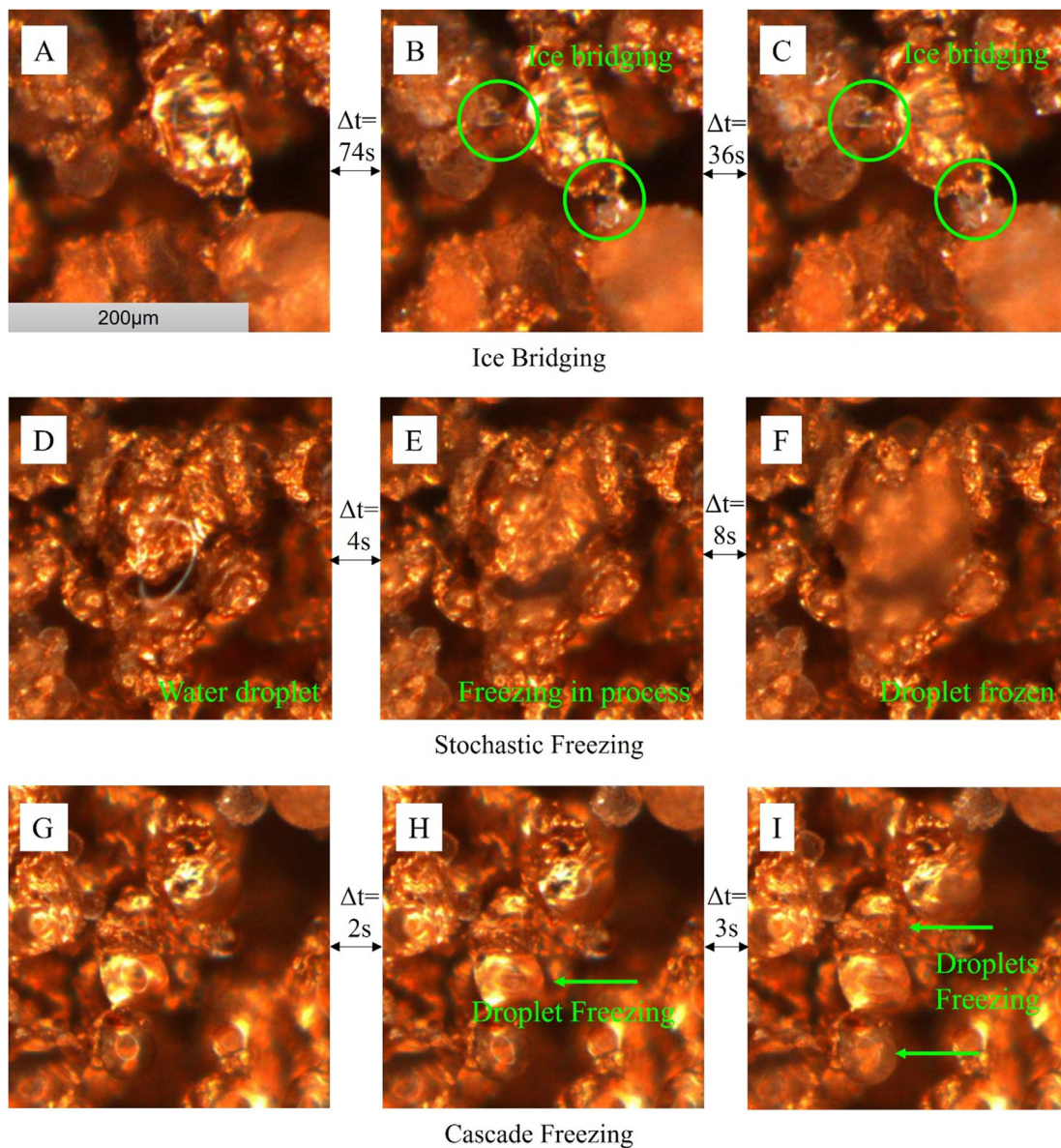
FIG. 5. The mechanisms of droplets freezing on the sintered wick. (a)–(c) Ice bridging; (d)–(f) A droplet freezing despite experiencing no interactions from the droplets surrounding it via stochastic freezing; the freezing process is observed by the loss of reflectance between (d) and (e) and loss of transmittance between (e) and (f); (g)–(i) Droplets freezing due to cascade freezing; the two additional droplets freeze within a second of the first and are seen in supplementary video. Multimedia views: https://doi.org/10.1063/5.0105412.3 ; https://doi.org/10.1063/5.0105412.4 ; https://doi.org/10.1063/5.0105412.5
