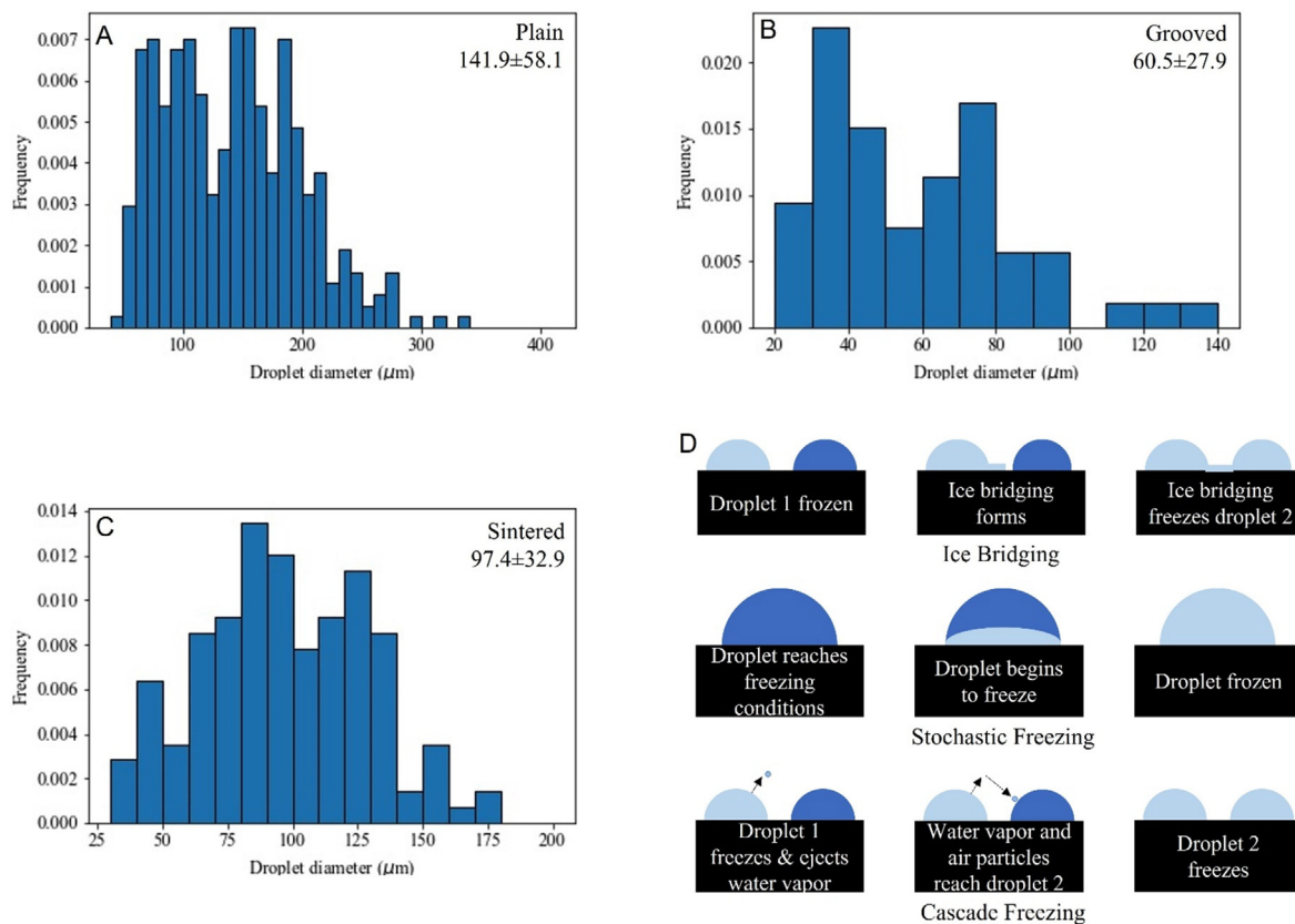
FIG. 2. Histograms of the size of frozen droplets from five experiments on the (a) Plain copper surface with a frozen droplet diameter range from 43.6 to 418.5 \mu\text{m} , (b) Grooved 2 with a frozen droplet diameter range from 24.9 to 142.7 \mu\text{m} , and (c) sintered 2 with a frozen droplet diameter range from 33.9 to 203.1 \mu\text{m} . (d) a schematic of three droplet freezing mechanisms, ice bridging, stochastic freezing, and cascade freezing.
