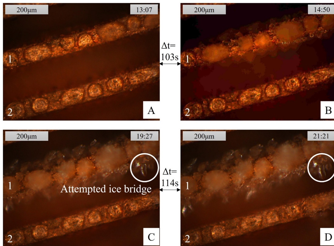
FIG. 4. Droplets freezing on the top of two grooves in a grooved wick (i.e., the portion of the groove furthest from the Peltier cooler). (a) The droplets have begun to freeze on one of the grooves, (b) the droplets on groove 1 are completely frozen, (c) almost 4.5 min after the droplets on groove 1 froze, the droplets on groove 2 remain as water, though the ice is attempting to reach out in the creation of an in-plane ice bridge, (d) a little under 5.5 min after the droplets on groove 1 are completely frozen, groove 2 begins to freeze, even though the ice has not bridged the gap between the grooves, additionally, the ice attempting to bridge stops growing without a water source. Multimedia view: https://doi.org/10.1063/5.0105412.2
