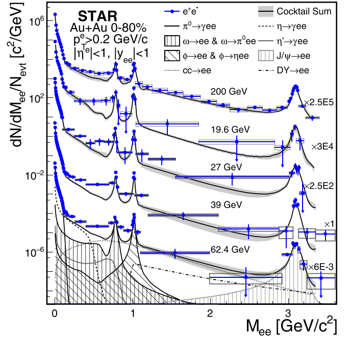
FIG. 1. Background subtracted dielectron invariant mass spectra within the STAR acceptance from \sqrt{s_{NN}} = 19.6, 27, 39, 62.4 , and 200 GeV 0–80% most-central Au + Au collisions. Errors bars and open boxes represent the statistical and systematic uncertainties in the measurements. The solid black curves represent the hadronic cocktail, with the gray bands representing the cocktail uncertainties. The curves underneath the \sqrt{s_{NN}} = 62.4 GeV hadronic cocktail curve and gray band represent the cocktail components at 62.4 GeV. For better presentation, the measurements and cocktail predictions are not listed in order by energy but have been scaled by factors 2.5 \times 10^5 , 3 \times 10^4 , 2.5 \times 10^2 , 1, and 6 \times 10^{-3} for results at \sqrt{s_{NN}} = 200, 19.6, 27, 39 , and 62.4 GeV, respectively.
