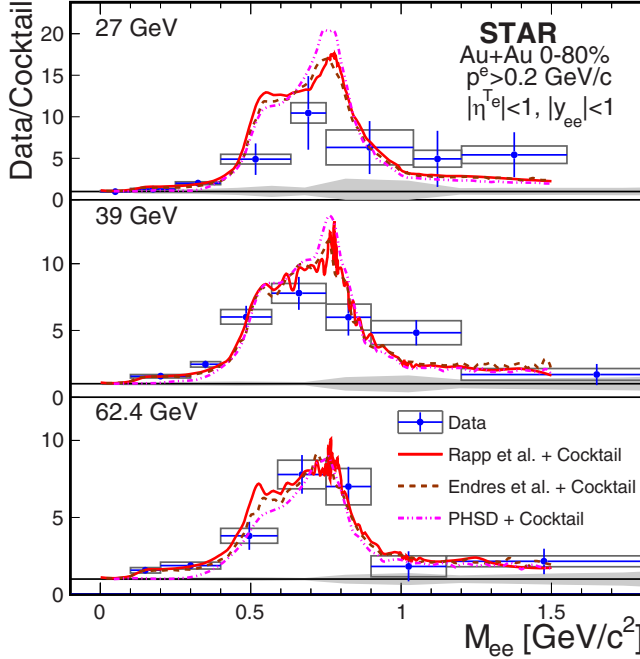
FIG. 2. The ratio of the invariant mass spectra to the cocktail with the \omega and \phi yields removed from both the data and cocktail. The gray area shows the cocktail uncertainties. Model calculations by Rapp et al. [13], Endres et al. [30], and PHSD [14,15] were separately added to the reference cocktail and compared to the reference cocktail, via ratios, as shown with the curves.
