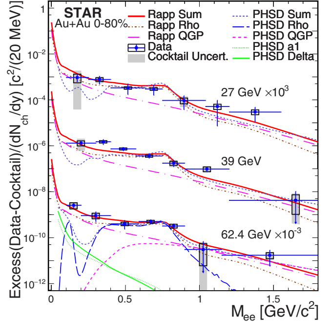
FIG. 3. Acceptance-corrected dielectron excess mass spectra, normalized by dN_{ch}/dy , for Au + Au collisions at \sqrt{s_{NN}} = 27, 39 , and 62.4 GeV. Model calculations (curves) [13–15] are compared with the excess spectra for each energy, as explained in the text. Individual components of the PHSD model calculations are only shown for Au + Au collisions at \sqrt{s_{NN}} = 62.4 GeV. The error bars, open boxes, and filled boxes indicate statistical, systematic, and cocktail uncertainties. A 6% uncertainty on the acceptance correction is not shown.
