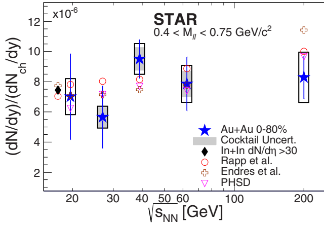
FIG. 4. Collision energy dependence of the integrated dilepton excess yields in 0.4 < M_{ll} < 0.75 GeV/ c^2 , normalized by dN_{ch}/dy . The closed markers represent the experimental measurements, while the open markers represent the calculations from Rapp et al. , Endres et al. , and PHSD. For measurements at \sqrt{s_{NN}} = 27, 39 , and 62.4 GeV, the open and filled (gray) boxes represent the systematic errors in the measurements and the cocktail uncertainties, respectively. The 6% uncertainty from the acceptance correction is not included. For measurements of minimum-bias, 0–80% central Au + Au collisions at \sqrt{s_{NN}} = 19.6 and 200 GeV, the open boxes represent the total systematic uncertainty in the measurements.
