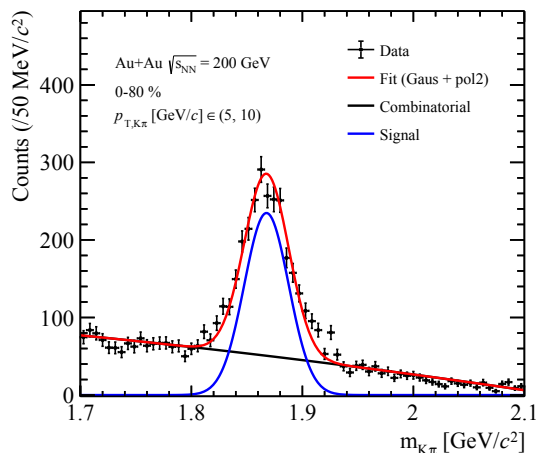
Fig. 1. (Color online) The invariant mass distribution of K\pi pairs with p_T \in (5, 10) GeV/ c . The unlike sign K\pi pair distribution (straight/black) is fit with a Gaussian plus second-order polynomial function (higher/red) to estimate the D^0(\bar{D}^0) yield. The signal after the removal of the background (lower/blue) is also shown.
