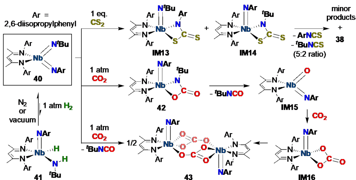
Scheme 12 1,2-Addition and [2+2] cycloaddition reactivity of asymmetric Nb bis(imido) complex 40.
