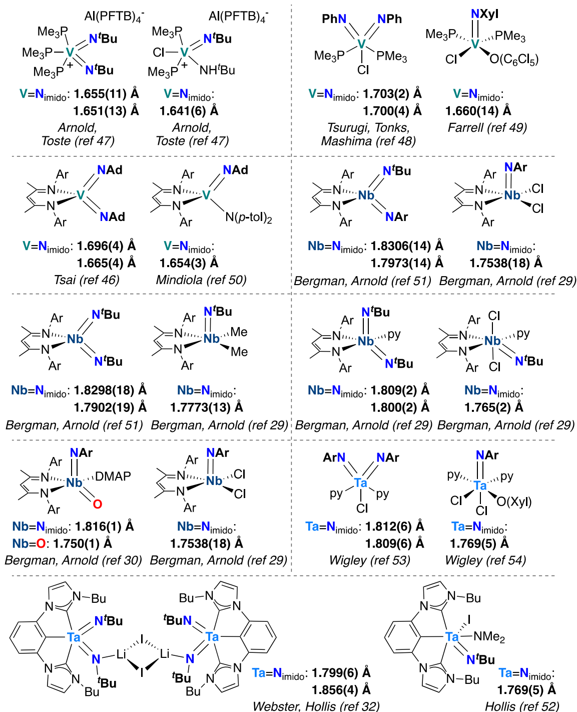
Figure 3 Crystallographically characterized pairs of closely related group 5 bis(imido) (or oxo-imido) and mono(imido) complexes, with \text{M}=\text{N}_{\text{imido}} (or \text{M}=\text{O} ) bond lengths in Å. Ar = 2,6-diisopropylphenyl.
