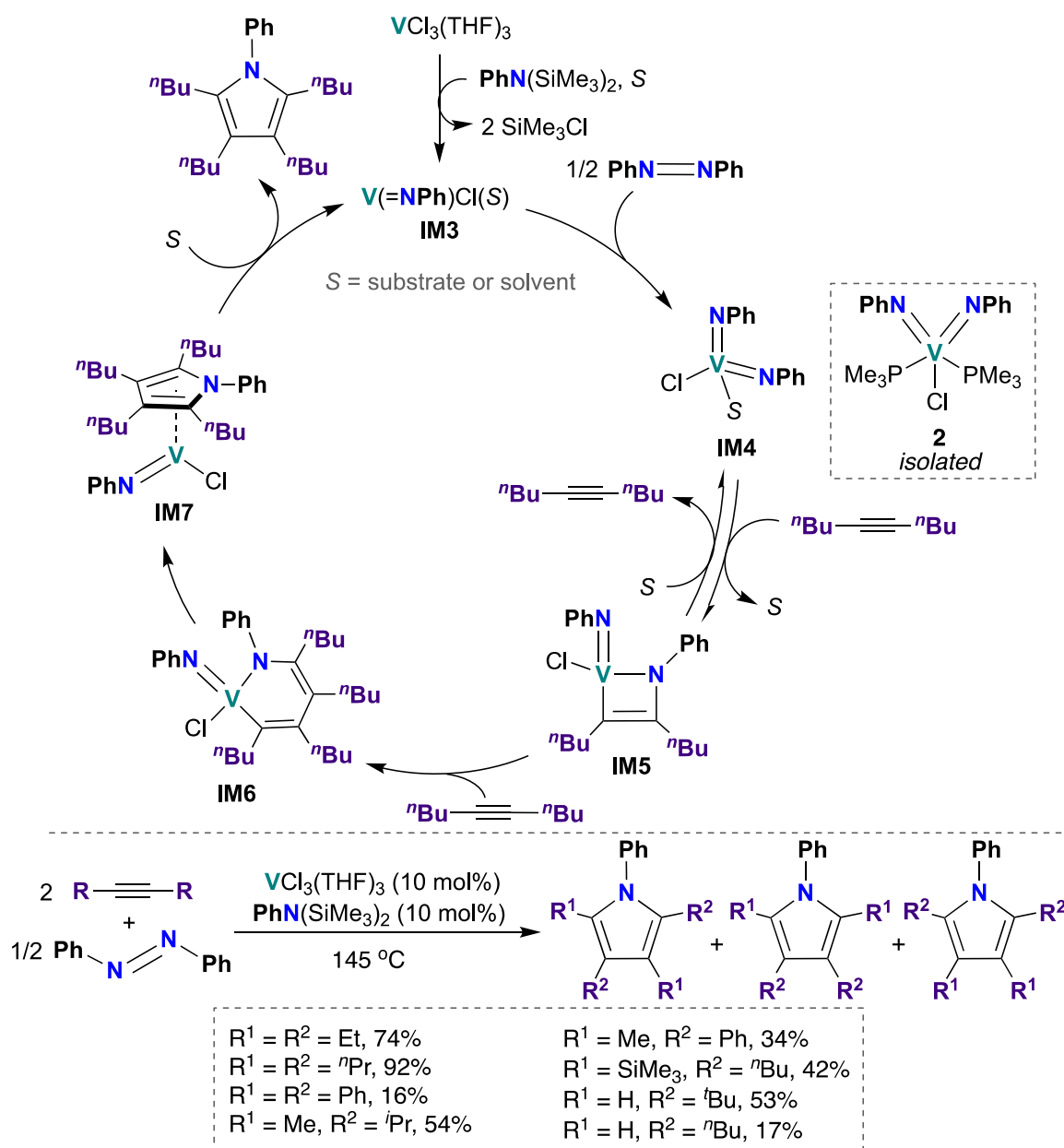
Scheme 2 V bis(imido)-catalyzed [2+2+1] coupling of alkynes and azobenzenes to give multisubstituted pyrroles.
