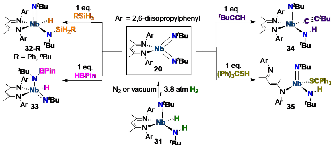
Scheme 11 1,2-Addition reactivity of Nb bis(imido) complex 20 toward element-hydrogen bonds.
