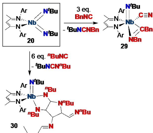
Scheme 10 Reactivity of Nb bis(imido) complex 20 with excess alkyl-substituted isocyanide.
