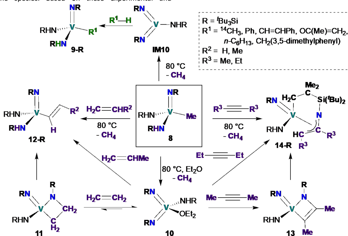
Scheme 4 1,2-addition and [2+2] cycloaddition reactivity of V bis(imido) complexes.
