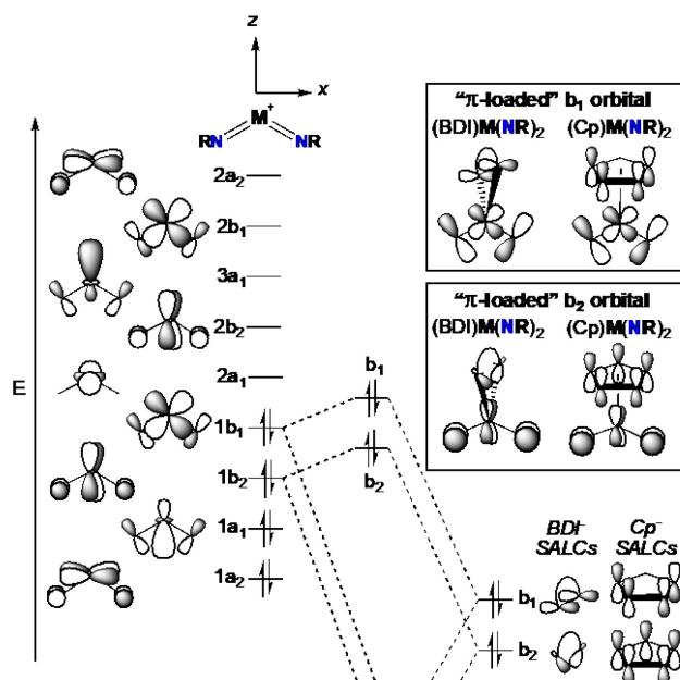
Figure 2 Molecular orbitals for the [M(NR)_2]^+ fragment (left, M = V, Nb, Ta ), selected symmetry adapted linear combinations (SALCs) of molecular orbitals for a cyclopentadienyl (Cp) ancillary ligand and a \beta -diketiminate (BDI) ancillary ligand (right), and relative energy and symmetry considerations for the combination of the [M(NR)_2]^+ fragment and a monoanionic, \pi -donor ligand (center). Relative energies of molecular orbitals are not drawn to scale.
