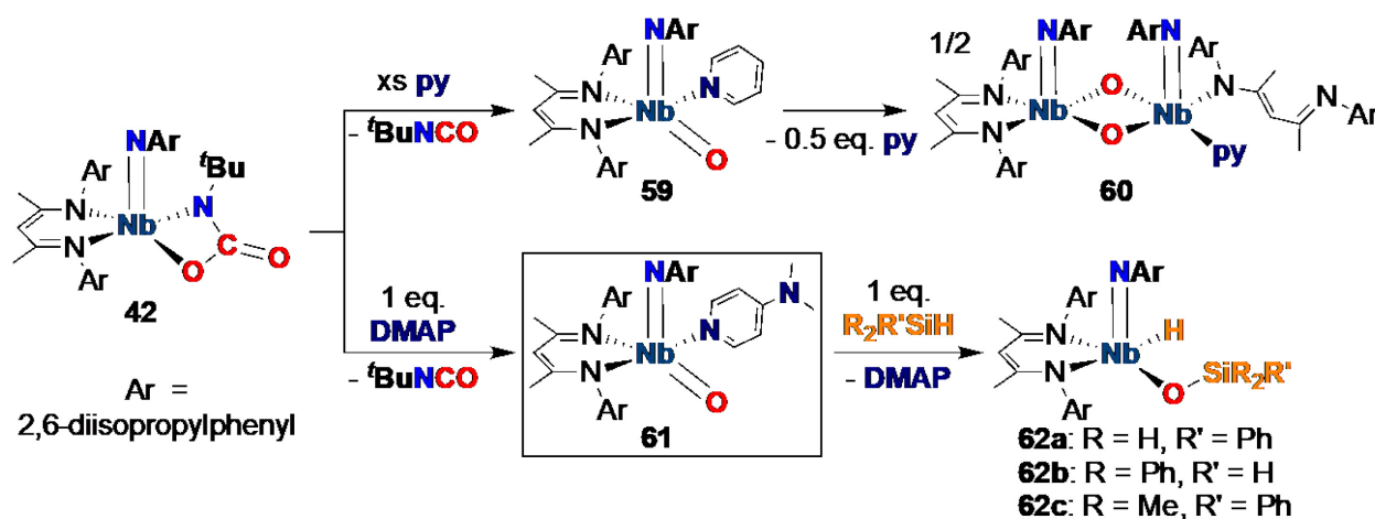
Scheme 18 Synthesis and 1,2-addition reactivity of \pi -loaded Nb oxo-imido complex 61.
