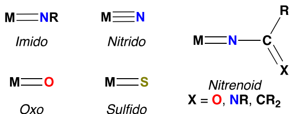
Figure 1 Common \pi -bonded metal-heteroatom species.
