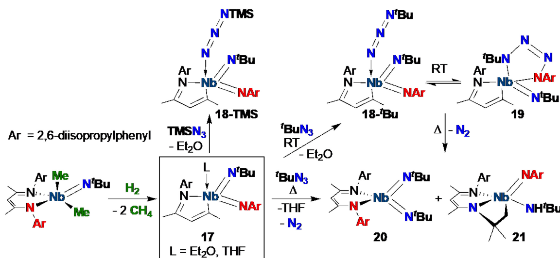
Scheme 6 Reactivity of a MAD-supported Nb bis(imido) complex with organic azides.
