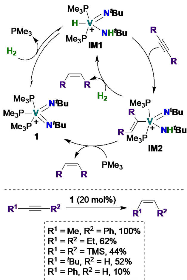
Scheme 1 V bis(imido)-catalyzed semihydrogenation of alkynes to Z-alkenes.
