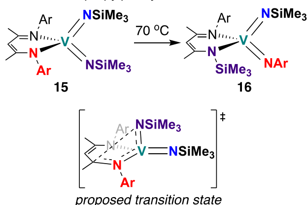
Scheme 7 Intramolecular ligand insertion reactivity of a V bis(imido) complex.
