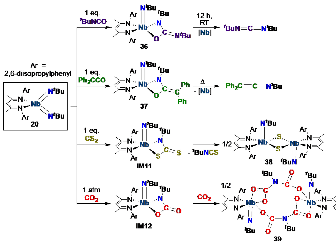
Scheme 13 [2+2] Cycloaddition reactivity of Nb bis(imido) complex 20 toward heteroallenes.
