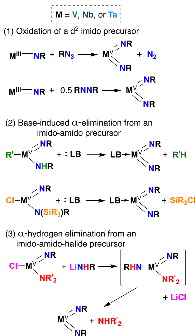
Figure 4 Synthetic routes to group 5 bis(imido) complexes.
