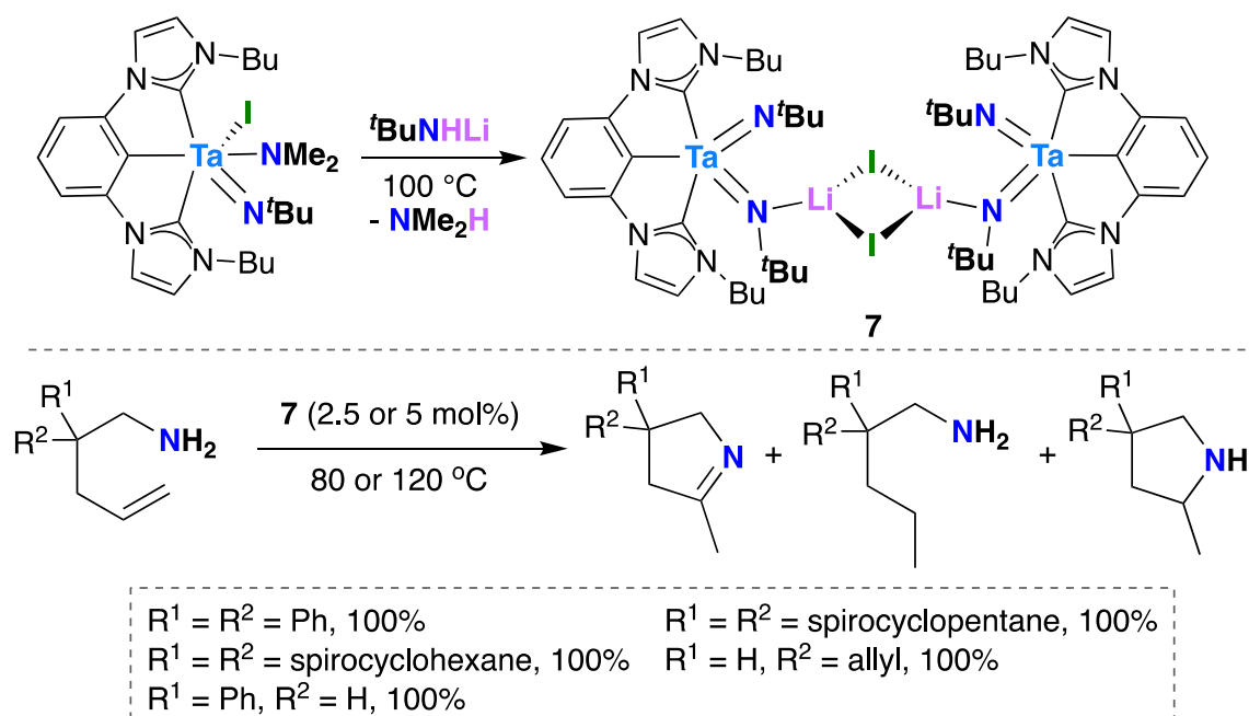
Scheme 5 Ta bis(imido)-catalyzed oxidative amination of alkenes to yield cyclic imines, cyclic amines, and hydrogenated substrate.
