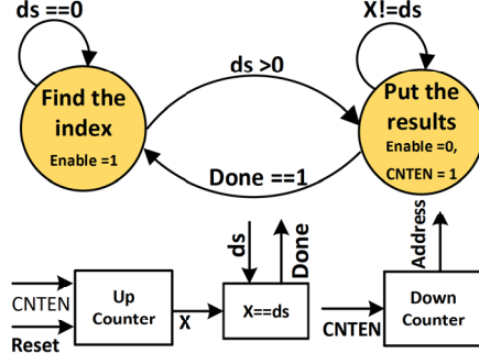
Fig. 3: Proposed Controller.
