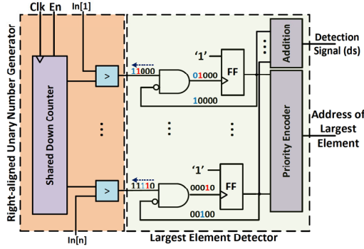
Fig. 2: Proposed Unary Sorting Engine.
