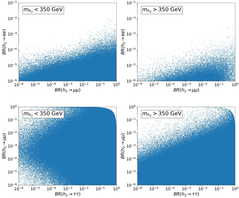
FIG. 2: These scatterplots show allowed points for h_2 decays. Results are shown for h_2 masses below 350 GeV and above that mass scale (at which point the \bar{t}t channel opens up). The upper figures plot ee and \mu\mu decays and the lower figures plot \mu\mu and \tau\tau decays. The decay branching ratio of the SM Higgs to \mu\mu is approximately 2 \times 10^{-4} .
