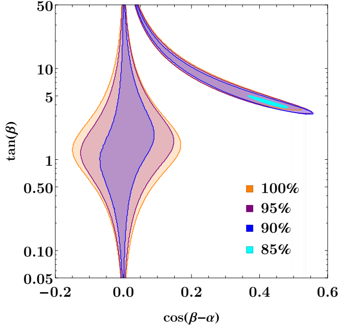
FIG. 1: Allowed regions in the \tan \beta - \cos(\beta - \alpha) plane, in the model without (q\tau) -( \mu e ) mixing, for different values of r \equiv (v_q^2 + v_\tau^2)^{1/2}/v , namely r = 1 in orange, r = 0.95 in purple, r = 0.90 in blue and r = 0.85 in cyan.
